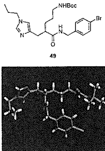
Figure 1. Single-crystal X-ray structure of 49 confirming the (2 S ) stereochemistry of 21.
