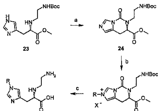
Scheme 2 a
