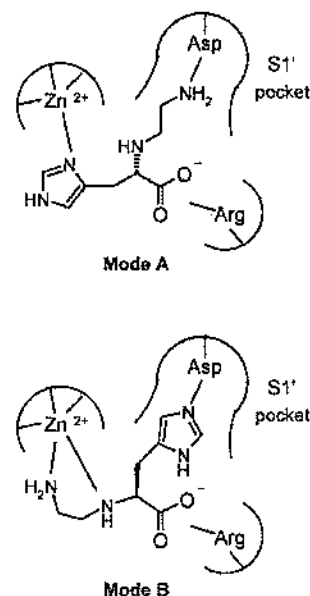
Figure 3. Schematic model of the binding site of TAFIa illustrating the possible binding modes of compound 8 .
