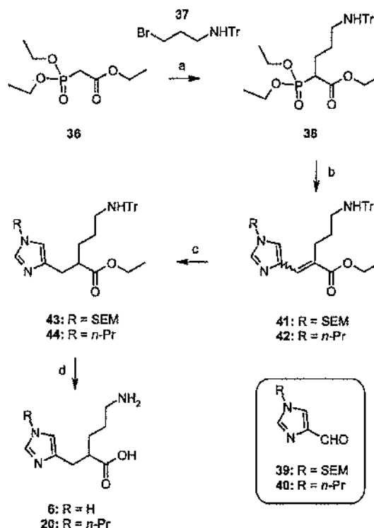
Scheme 3 a
