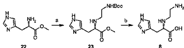
Scheme 1 a
