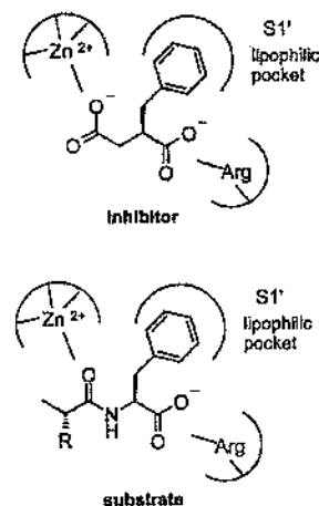
Figure 2. Schematic model of the binding site of CPA illustrating the proposed binding mode of the inhibitor and peptide substrate.
