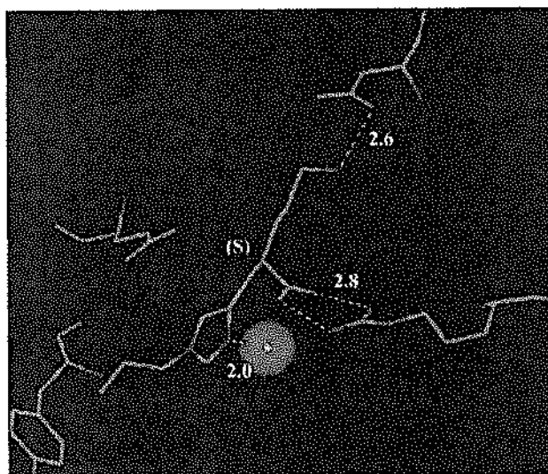
Figure 5. Structure of 21 in porcine pCPB showing key interactions and distances (Å). The catalytic zinc in this representation is displayed as a purple sphere.
