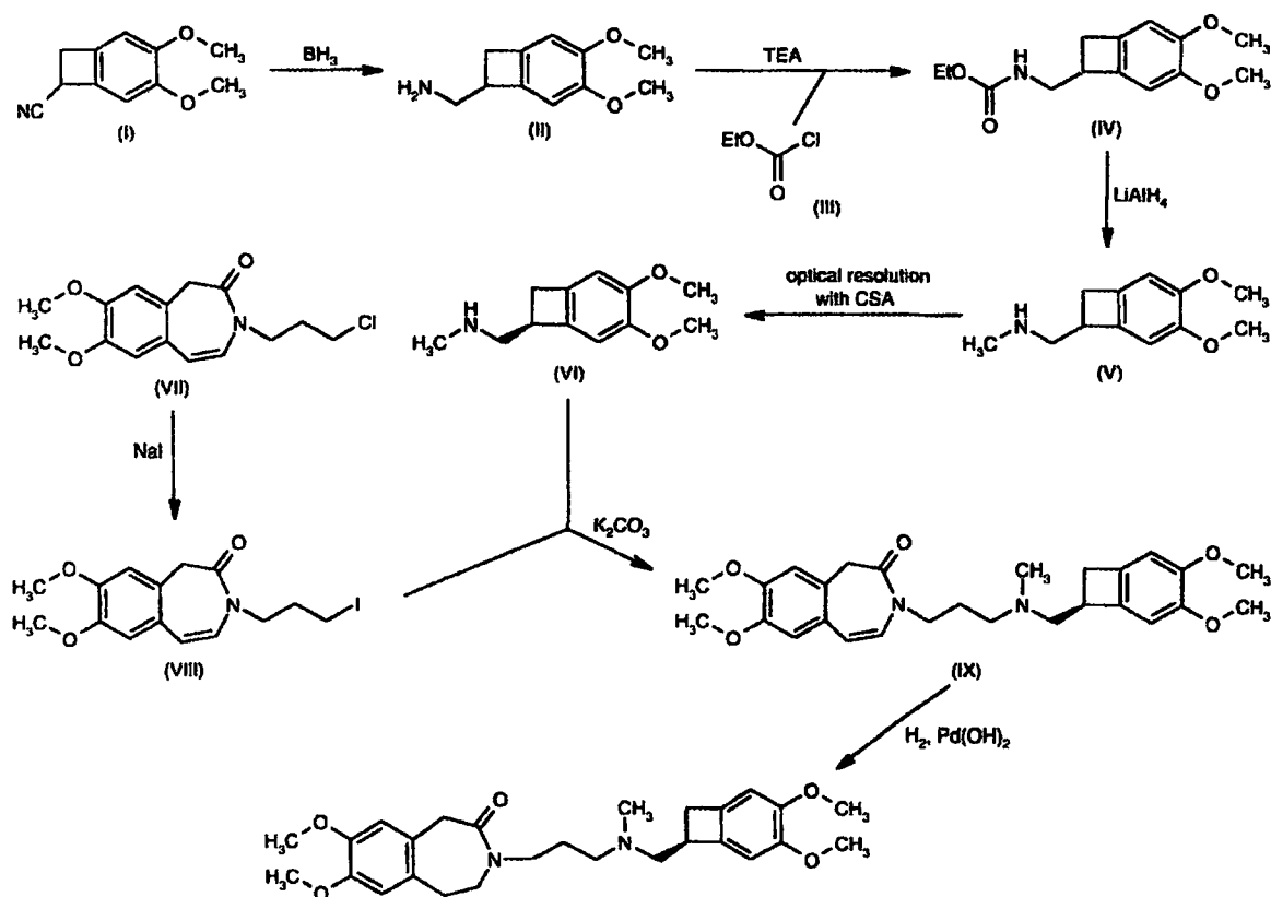
Scheme 1: Synthesis of Ivabradine
