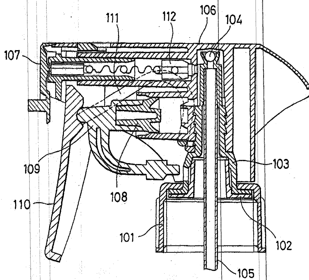
FIG.9 PRIOR ART
