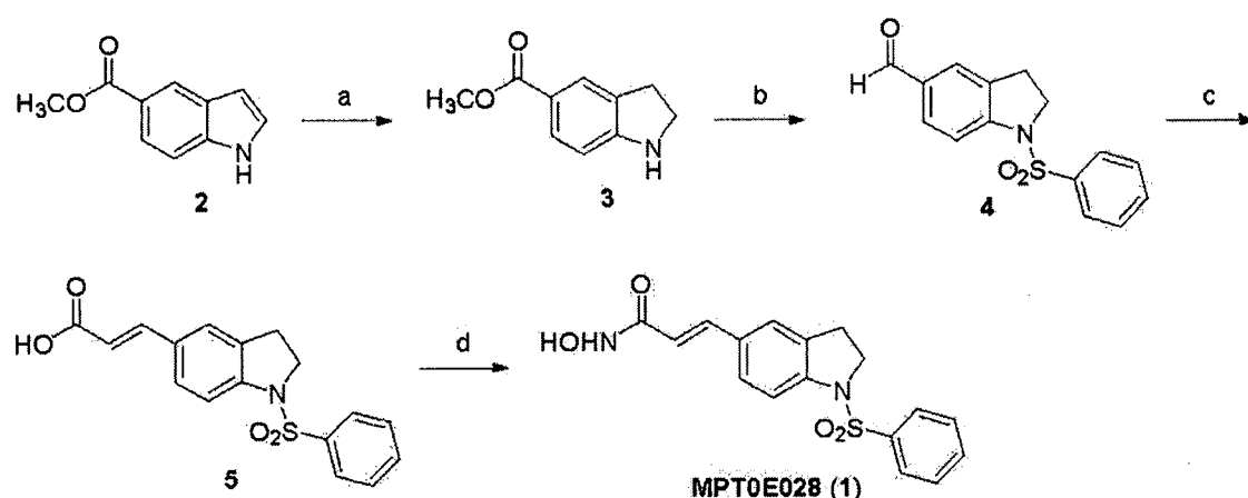
Figure 1. The synthesis of MPT0E028. Reagents and conditions. (a) NaBH 3 CN, AcOH, 0°C–r.t.; (b) (i) benzenesulfonyl chloride, pyridine, reflux; (ii) LiAlH 4 , THF, 0°C–r.t.; (iii) pyridinium dichromate (PDC), molecular sieves, CH 2 Cl 2 , r.t.; (c) (i) methyl(triphenylphosphoryl)acetate, CH 2 Cl 2 , r.t.; (ii) 1 M LiOH(aq), dioxane, 40°C; (d) (i) NH 2 OTHP, PYBOP, Et 3 N, DMF, r.t.; (iii) trifluoroacetic acid, CH 3 OH, r.t. Abbreviations: NaBH 3 CN, sodium cyanoborohydride; AcOH, acetyl acid; LiAlH 4 (LAH), lithium aluminium hydride; THF, tetrahydrofuran; PDC, pyridinium dichromate; NH 2 OTHP, O-(tetrahydro-2H-pyran-2-yl)hydroxylamine; PYBOP, benzotriazol-1-yl-oxytripyrrolidinophosphonium hexafluorophosphate; Et 3 N, triethylamine; DMF, dimethylformamide; TFA, trifluoroacetic acid. doi:10.1371/journal.pone.0043645.g001
