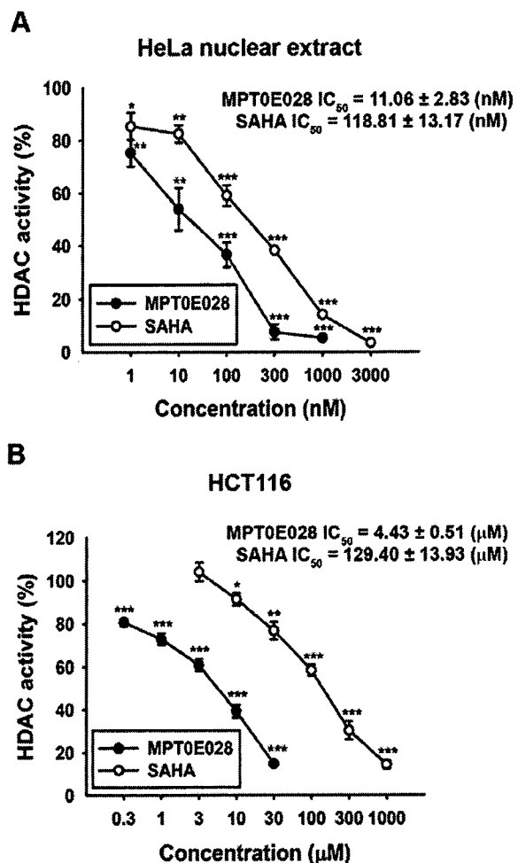
Figure 3. Inhibition of HDACs activity by MPT0E028 and SAHA. (A) Inhibition of HDACs activity in HeLa nuclear extracts. Data were expressed as the mean of at least 3 independent experiments. (B) Inhibition of total HDAC activity by MPT0E028 and SAHA. HCT116 cells were treated with the indicated concentrations of MPT0E028 and SAHA for 24 h, and the nuclear proteins were isolated to determine the inhibition of total HDAC enzyme activity. Data are expressed as the mean ± S.E.M. of at least 3 independent experiments.
