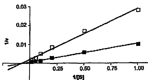
Figure 4. Lineweaver-Burke analysis of the hydrolysis of [ ^3\text{H} ]anandamide (1–100 \mu\text{M} ) by rat brain membranes in the absence (■) or presence (□) of compound 7 (1 \mu\text{M} ). Results are from one experiment, representative of five in which maximal velocities ( V_{\text{max}} ) for [ ^3\text{H} ]anandamide hydrolysis were 2271 \pm 477 pmol/(min·mg) protein in control samples and 703 \pm 188 pmol/(min·mg) protein in the presence of compound 7 ( p < 0.05 ). Michaelis-Menten constants ( K_M ) were 9.3 \pm 2.3 \mu\text{M} in control samples and 10.2 \pm 3.3 \mu\text{M} in the presence of compound 7 ( p > 0.05 , Student's t test; n = 5 ).
