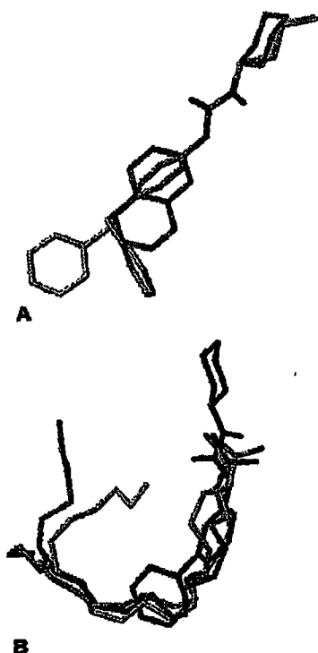
Figure 5. (A) Representation of minimum energy conformations of 22 (green carbons) and 7 (white carbons, in gauche and anti conformations) after superposition of the carbamate group. (B) Superposition of the biphenyl moiety of 9i (orange carbons) to the lipophilic chain of arachidonic acid, cocrystallized with adipocyte lipid-binding protein (white carbons), COX-1 (yellow carbons), or COX-2 (green carbons).
