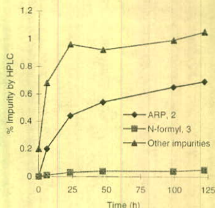
Figure 3—Spray-dried lactose and fluoxetine HCl at 85 °C.
