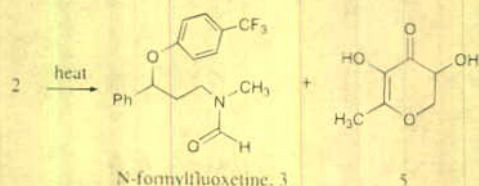
Scheme 3—Decomposition of ARP, 2
