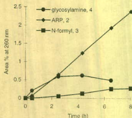
Figure 1—HPLC data for the reaction of fluoxetine HCl, lactose, and KOH at pH* 8.0, 60 °C in aqueous ethanol.
