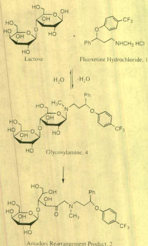
Scheme 2—Maillard reaction of lactose and fluoxetine HCl.
