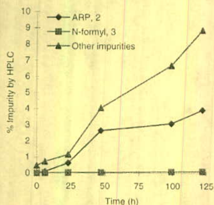
Figure 6—Generic N, a fluoxetine HCl/lactose capsule at 85 °C.
