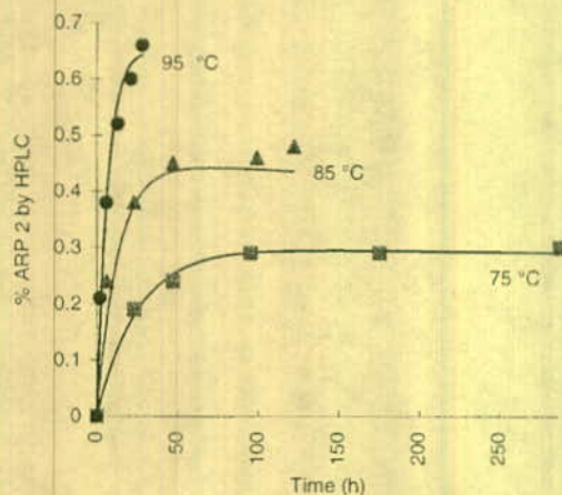
Figure 5—Formation of ARP, 2, from solid-phase mixtures of lactose monohydrate, fluoxetine HCl, and magnesium stearate. Points are experimental; lines are from eq 2.
