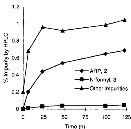
Figure 3—Spray-dried lactose and fluoxetine HCl at 85 °C.
