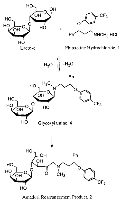
Scheme 2—Maillard reaction of lactose and fluoxetine HCl.
