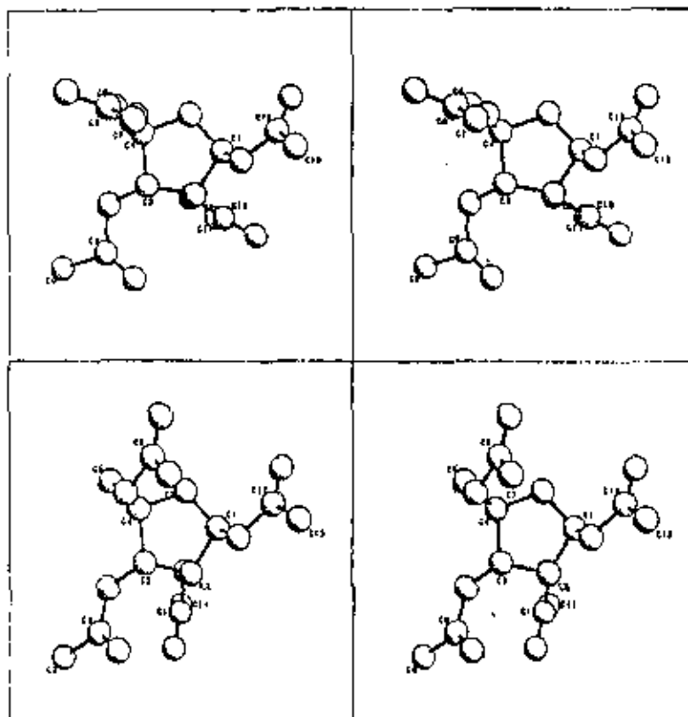
Figure 2. Stereoviews of the two forms of I. In both cases the view is on the planes of C1—O—C4 of the furanose ring: upper, monoclinic A form, lower, orthorhombic B form. For clarity, only carbon atoms are labeled.
