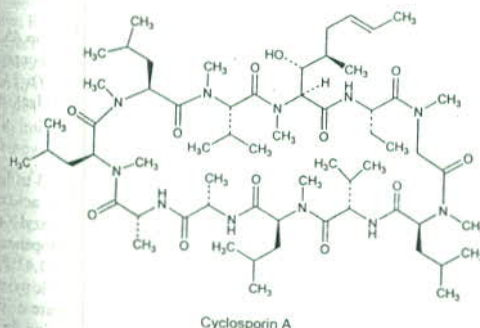
Cyclosporin A
