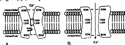
Fig. (3). The ion channel pore of the \alpha 7 receptor. (A) The charged residues in the extracellular ring involved in ion conductance, and those that form the ion selectivity filter on the intracellular side are labeled. Valine-252 and leucine-248 form the hydrophobic gate at the middle of the membrane. (B) Upon activation, a quaternary twist of the subunits opens the gate and allows the passage of cations.
