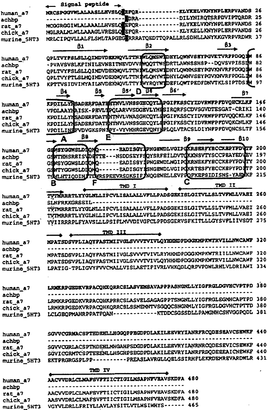
Fig. (1). Sequence of the human α7 nAChR compared with the α7 sequences from rat and chicken, and the sequence of the AChBP and murine 5HT 3 receptor. All are members of the ligand gated ion channel (LGIC) superfamily. The sequence alignments are based on a multi-sequence ClustalX alignment [187]. The first numbered residue in each sequence is highlighted in green. The putative binding loops, β strands and transmembrane domains are indicated. Loops A, B and C from the positive face of the LBD are indicated in red, and loops D, E and F from the negative face are indicated in blue. The β strands are numbered according to the AChBP crystal structure determination [2]. The conserved valine at position 202 is highlighted in yellow.
