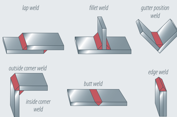
Different weld configurations
