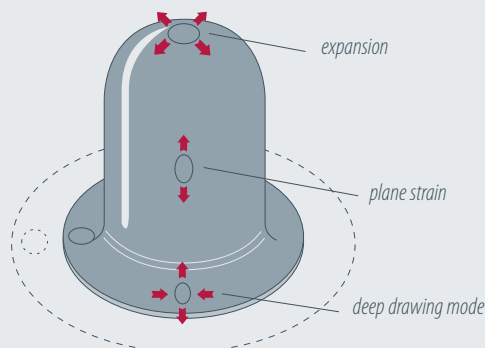
Different deformation modes in a drawn component
