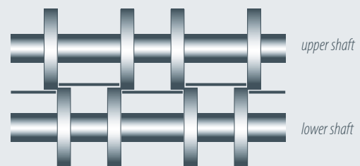
Symmetrical mounting of slitting blades
