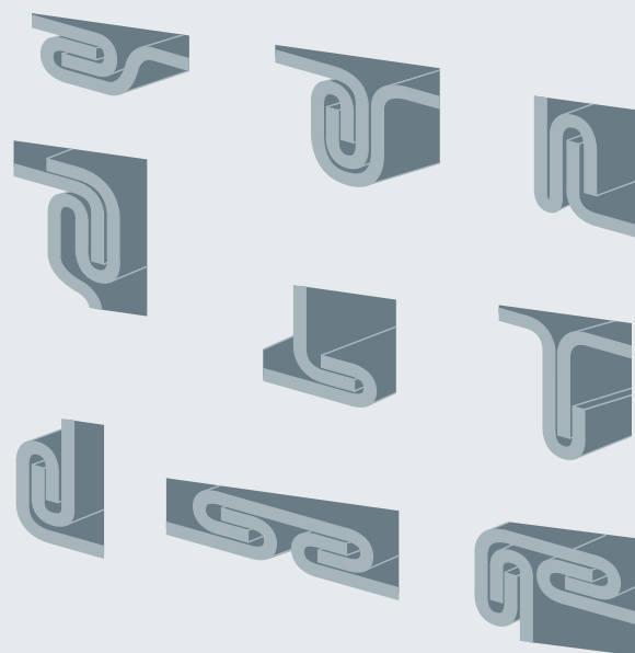
Different single and double lock seams
