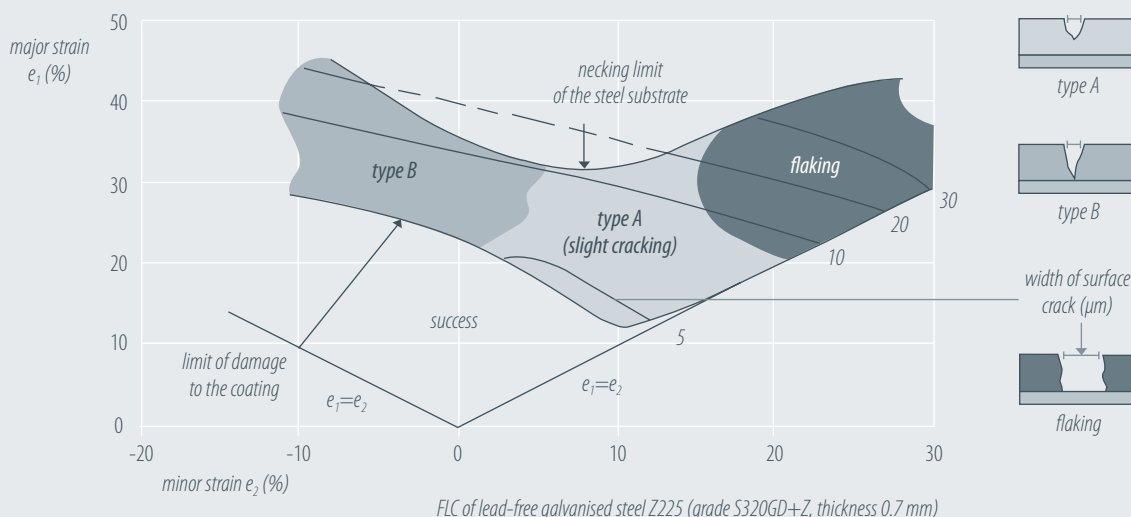
Different deformation modes in a drawn component
