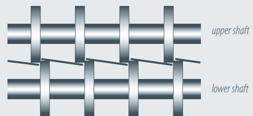
Non-symmetrical mounting of slitting blades
