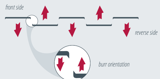
Burr orientation after slitting
