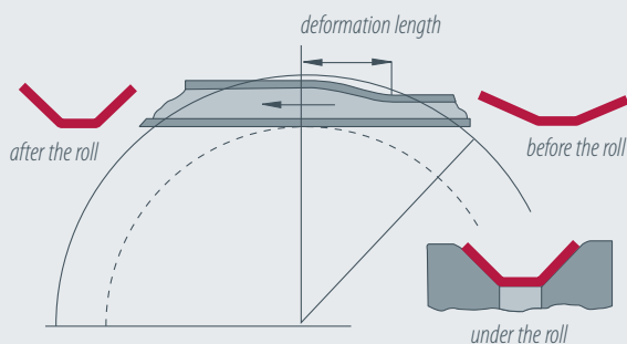
The influence of roll diameter
