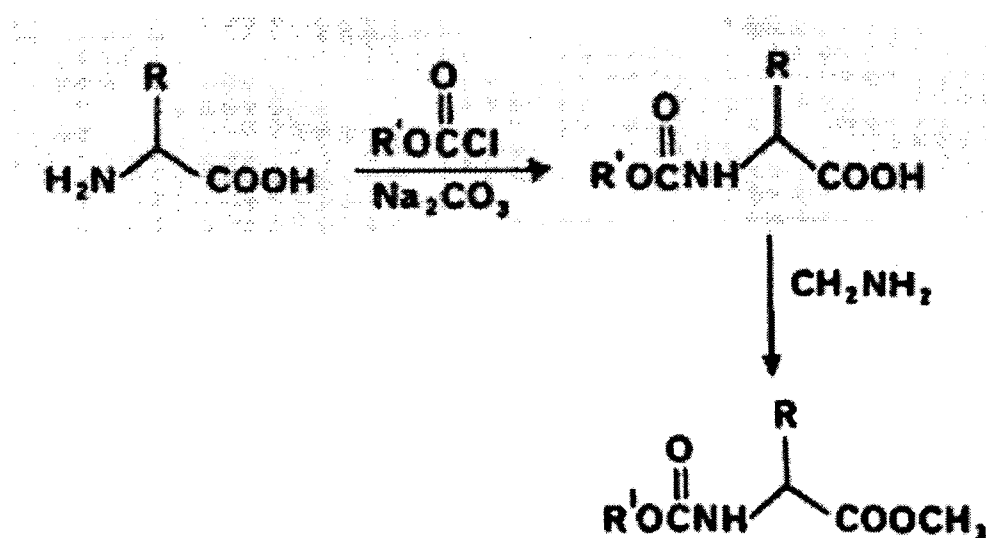
Fig. 5. Derivatization of amino acids by alkoxy carbonylation followed by esterification.
