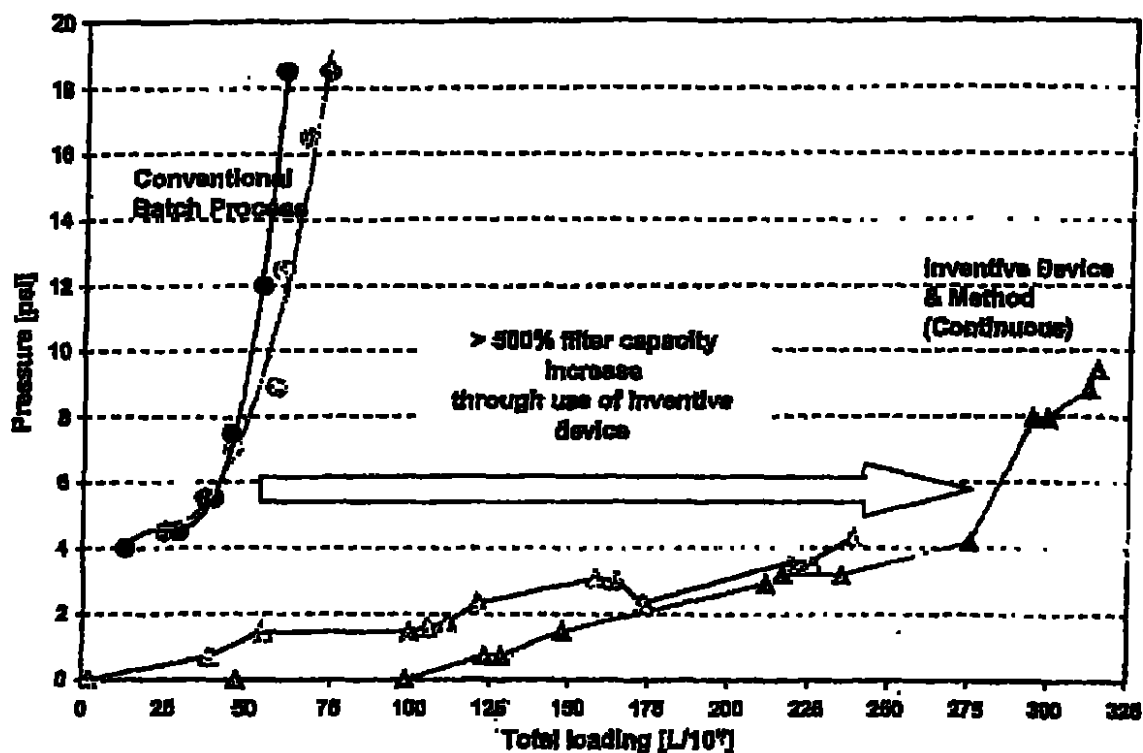
Figure 3: Example comparison of total load capacities per 10" of filter capsule for conventional batch process and embodiment of inventive device and method for continuous particle removal (integrated continuous filtration process) using identical commercial filter capsules. Example method producing recombinant blood coagulation Factor VIII shown.
