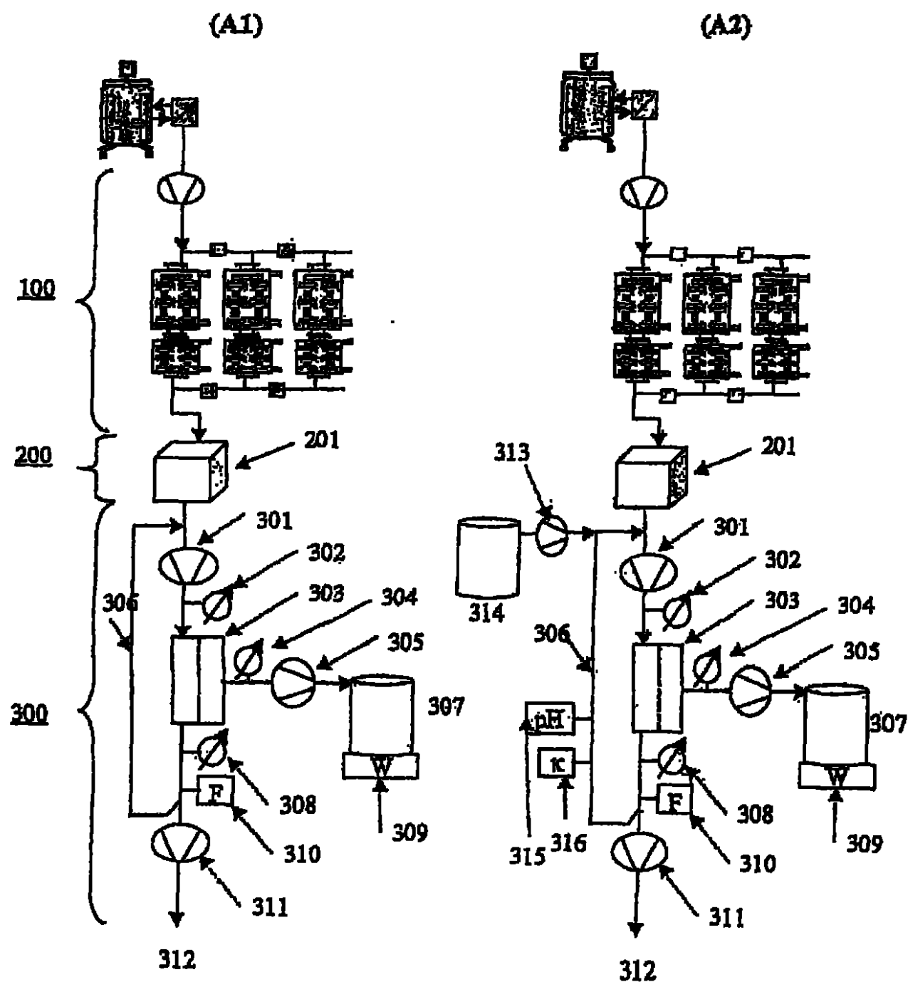
Figure 3: Schematic representation of 2 embodiments of inventive device A for continuous, integrated and sterile manufacturing. Schematic of embodiment A1 shown on left hand side and schematic of embodiment A2 shown on right hand side.
