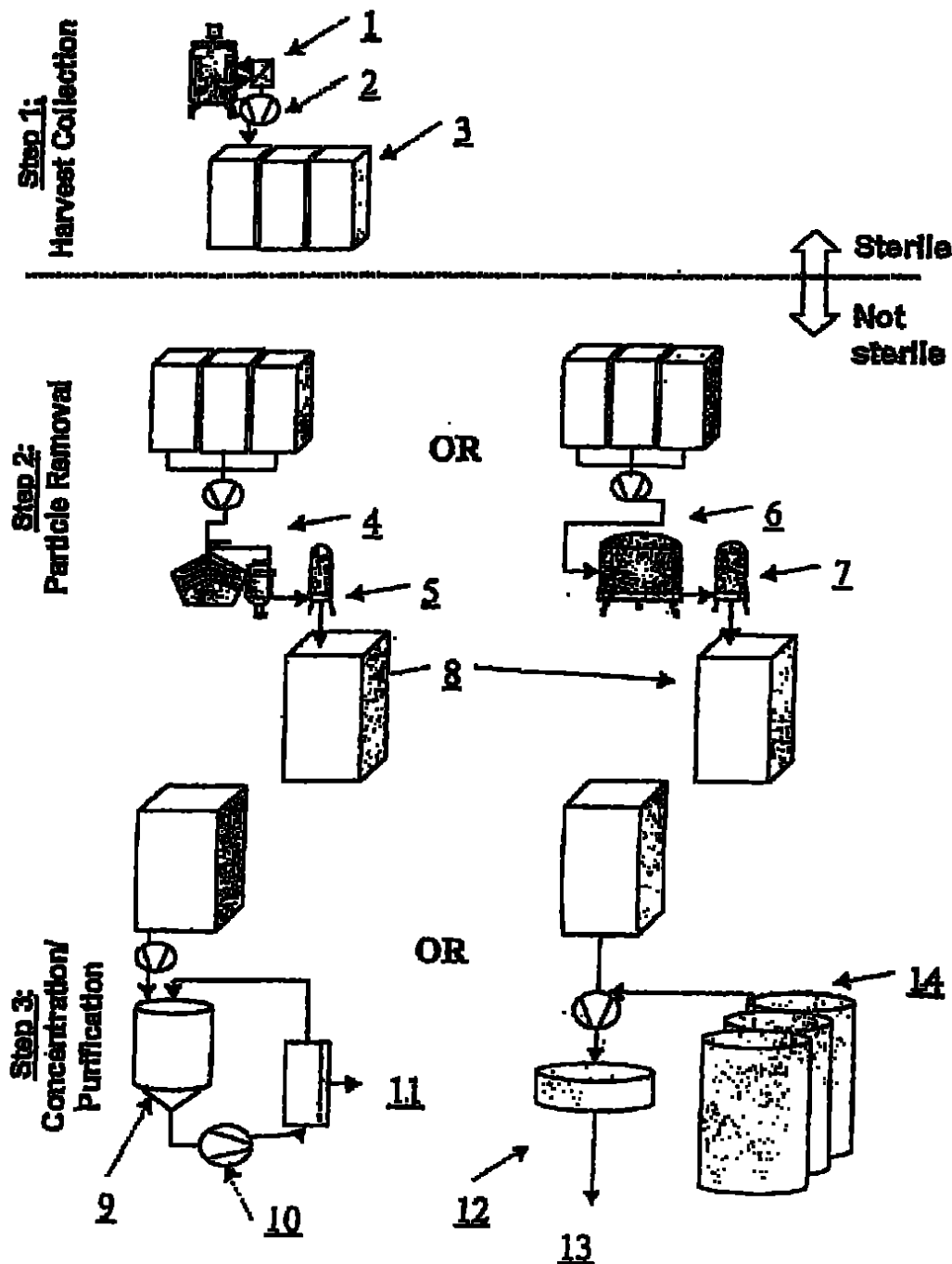
Figure 1: Schematic of conventional continuous perfusion process followed by 3 physically and logically segregated isolation process steps (batch harvest collection, batch particle removal and batch concentration/purification)
