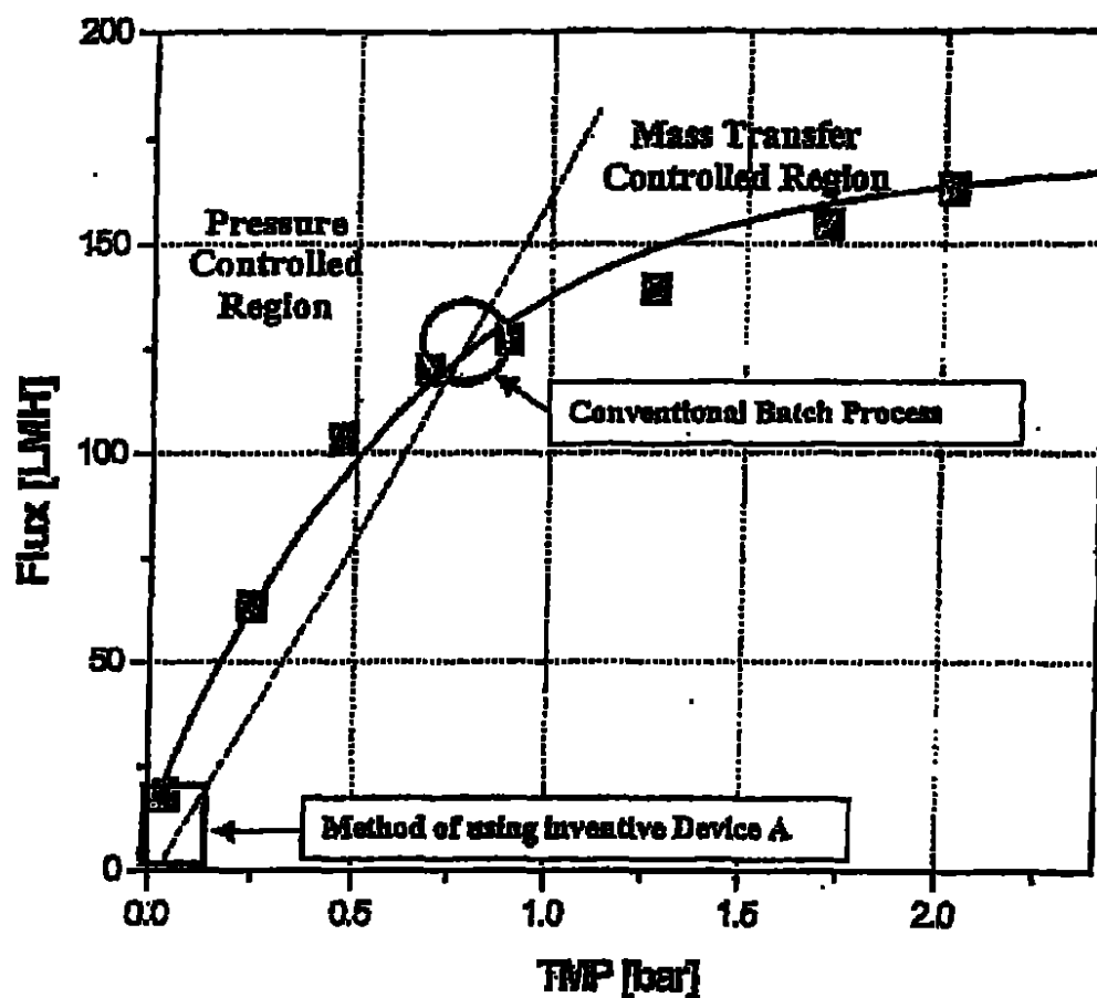
Figure 2: Example of pressure-flux curve (specific permeate flux in LMH = liters/hour/m 2 over transmembrane pressure) and determination of operation point. The circle shows the typical operation point that will be adjusted via the TMP for conventional batch processes. The rectangle shows the operational region that will be adjusted via the permeate pump as per the method of using the inventive device A.
