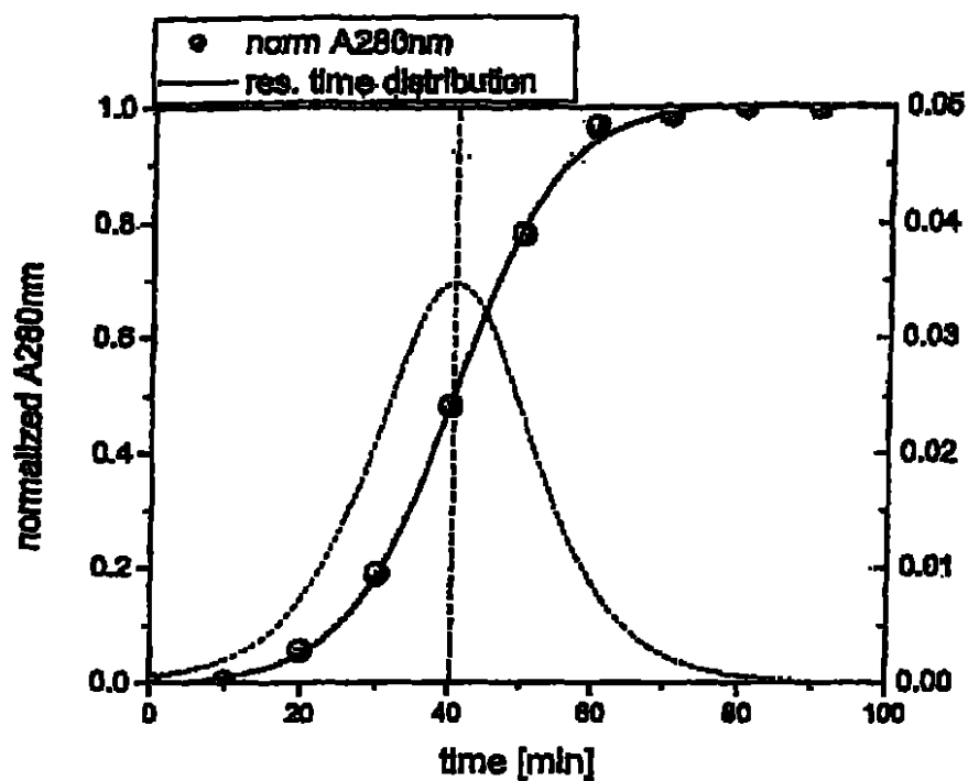
Figure 1A: Example of residence time distribution and mean residence time of integrated continuous UF system (300) as per method of using inventive device A. Measured for disposable continuous system with 290 cm 2 module (62.5 cm length), 120 LMH crossflow, 0.2 LMH retentate flow, 2 LMH permeate flow.
