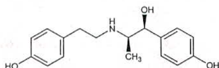
Relative stereochemistry
