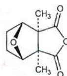
Relative stereochemistry
