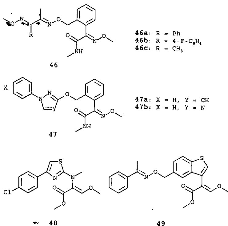
Scheme 14. Examples of strobilurins with variations of the side chain and aromatic bridge.
