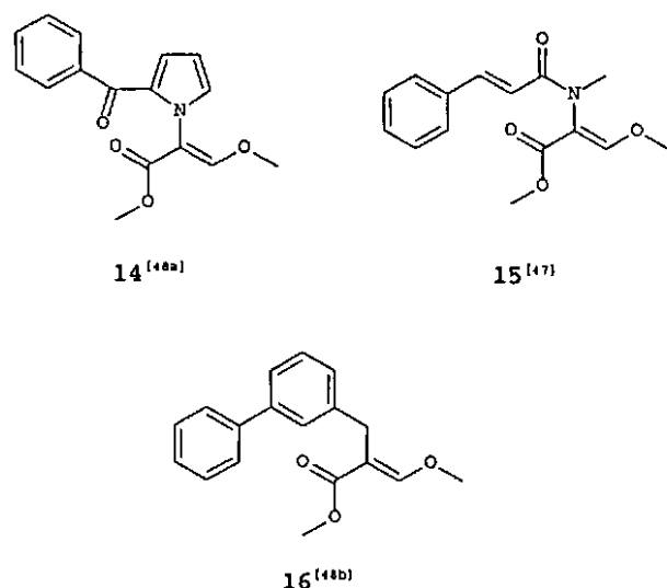
Scheme 7. Stabilized, active strobilurin variants from the early phase of the lead structure optimization at Zeneca. [45c]
