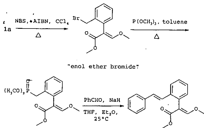
Scheme 3. Synthesis of the enol ether stilbene 7a . [24, 29a] AIBN = 2,2'-azobisisobutyronitrile, NBS = N -bromosuccinimide.
