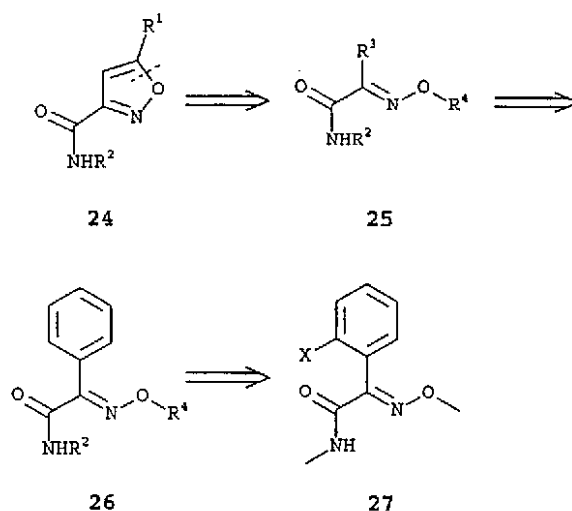
Scheme 10. Steps in Shionogi's sequence of thoughts for the synthesis of oxime ether amides 27. [63]
