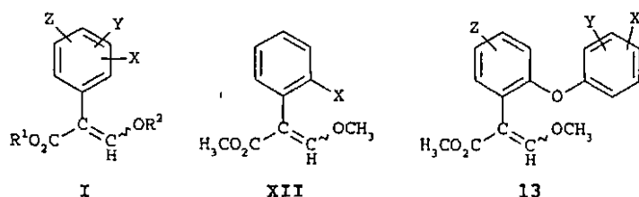
Scheme 6. Formulae from the claims in the ICI patent application for enol ether strobilurins [41] . See text for details.
