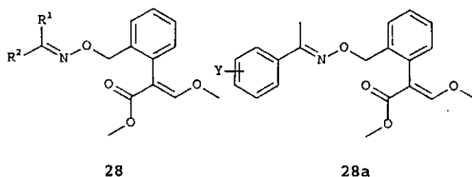
28b: R^1 = \text{CH}_3 , R^2 = \text{heteroaryl}
