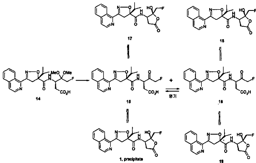
Reaction Scheme 3
