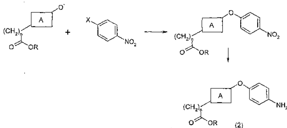
Scheme 6
