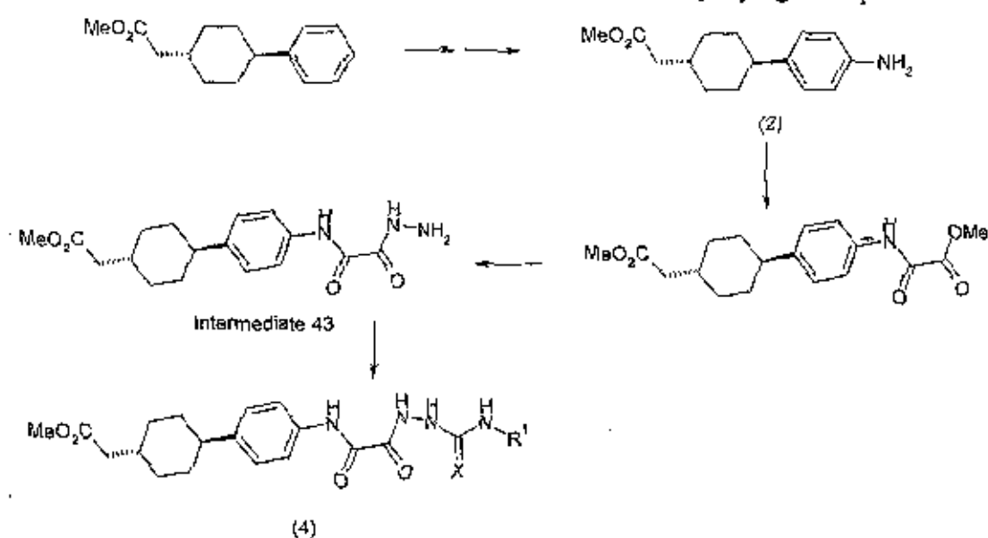
Scheme 4
