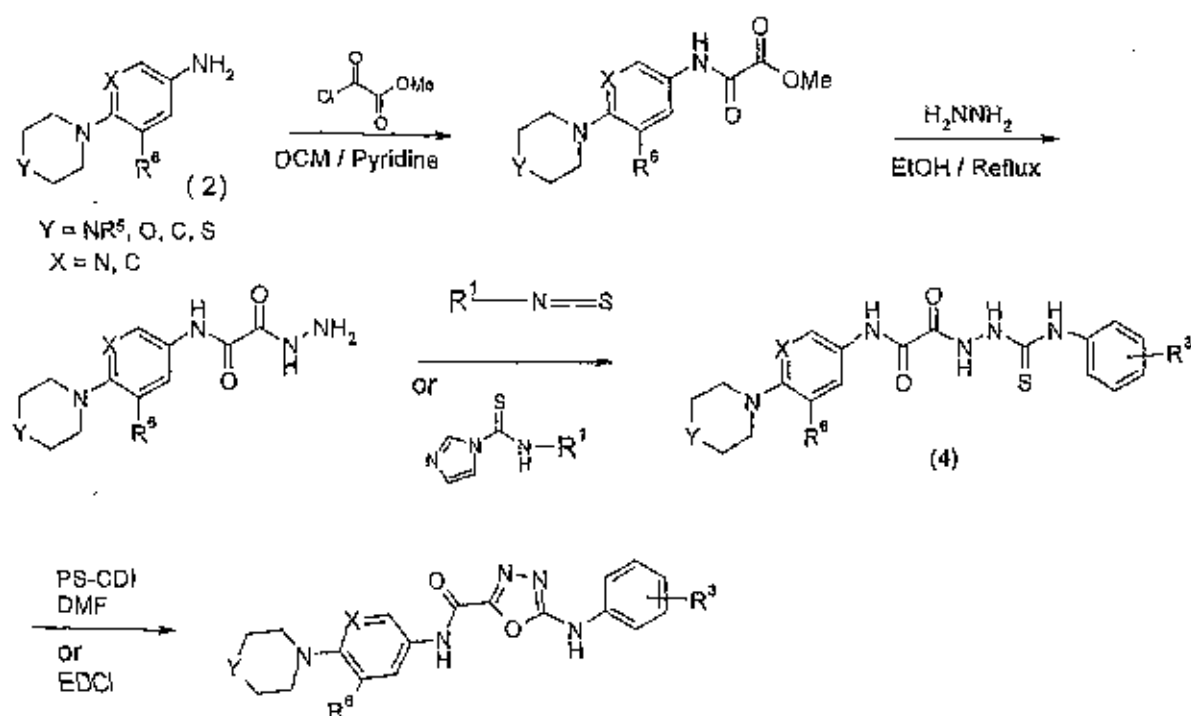
Scheme 7
