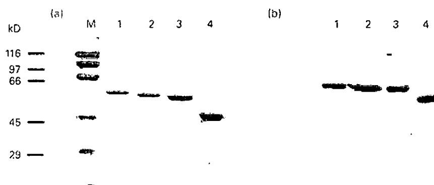
Fig. 3. Reactivity of viscero-cutaneous leishmaniasis (VCL) sera against all four core histones of Leishmania infantum . One microgram of the following recombinant proteins was loaded on 10% SDS-PAGE gels: rLiH2A (lane 1), rLiH2B (lane 2), rLiH3 (lane 3), and rLiH4-Nt (lane 4). Lane M contains the molecular weight markers. (a) Coomassie blue staining of the gel. (b) An equivalent gel was blotted to a nitrocellulose filter and probed with a pool of six VCL sera (1:100 dilution).
