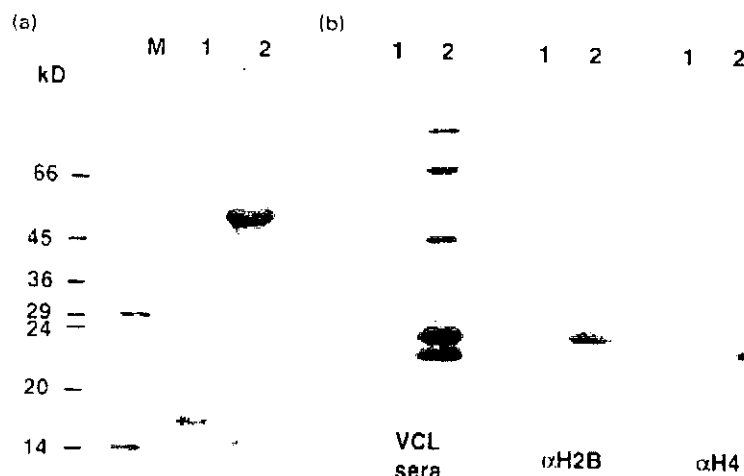
Fig. 2. Specificity of anti-histone antibodies present in viscerocutaneous leishmaniasis (VCL) sera. Calf thymus histone (6 µg; lane 1) and 20 µg of Leishmania infantum nuclear protein extracts (lane 2) were electrophoresed on linear 10–14% gradient SDS-PAGE gels. (a) Coomassie blue staining of the gel. Molecular weight markers are shown in kD (lane M). (b) Equivalent gels were blotted and probed either with a pool of six VCL sera (panel VCL sera), with the affinity-purified anti-H2B antibody fraction of VCL sera (panel αH2B), or with the affinity-purified anti-H4 antibody fraction of VCL sera (panel αH4).
