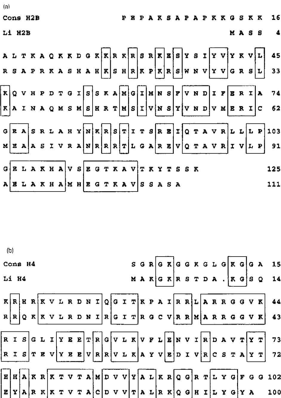
Fig. 1. Amino acid sequence alignment of Leishmania infantum histones H2B (a) and H4 (b) with consensus sequences for histones H2B and H4 (Cons [20]). Identical residues are boxed. A gap (indicated by a dot) has been introduced in the Leishmania histone H4 sequence (LiH4) to maximize the alignment.
