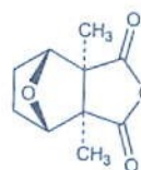
Relative stereochemistry
