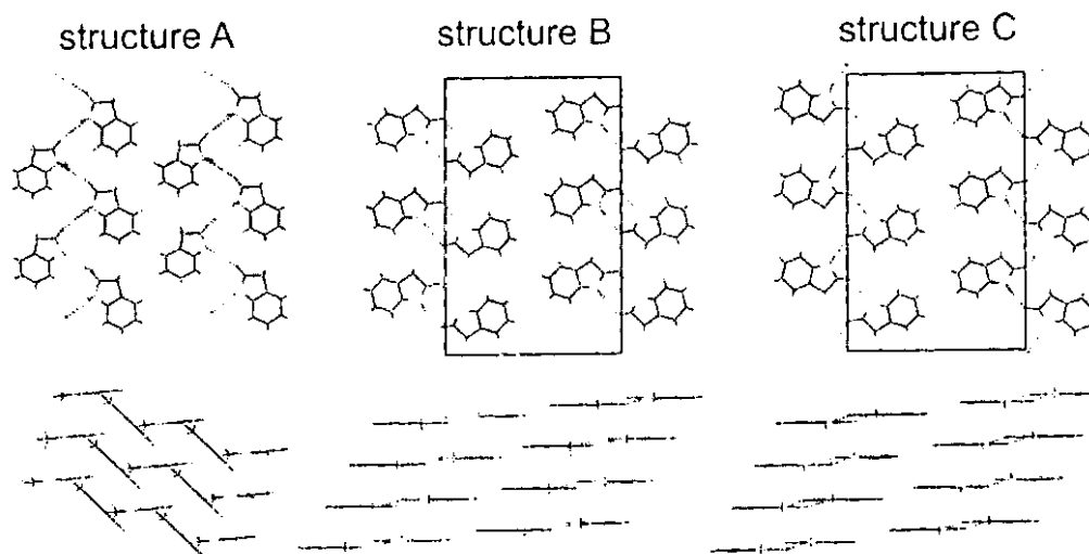
Figure 6. Hydrogen bonding (top) and stacking (bottom) in structures A, B, and C for 5-fluoro-2-oxindole. Grey boxes are included to highlight the areas of similar packing between structures B and C.
