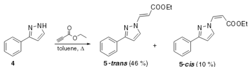
Scheme 2: condensation reaction of pyrazole 4 with ethyl propiolate
