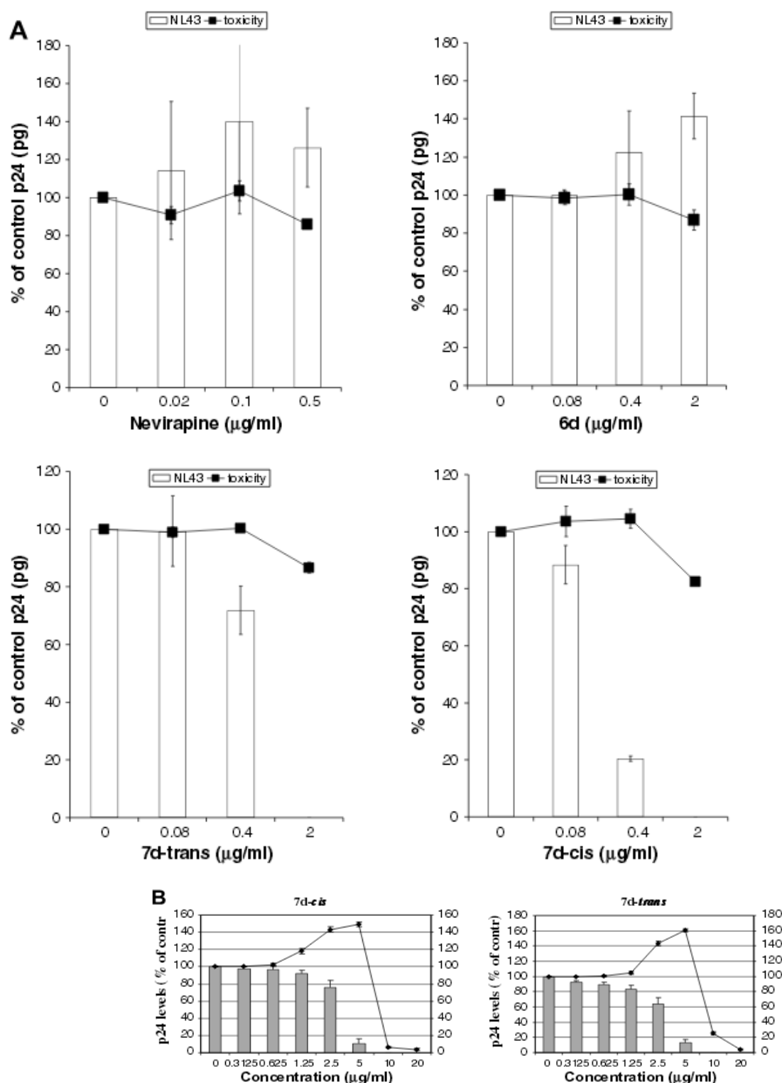
Figure 5. Inhibitory effects of 3-(5-phenyltetrazol-2-yl)acrylic acid ethyl esters on the release of infectious HIV-1 progeny (virus yield), p24 production (bars), in the supernatants of (A) transfected 293T cells or (B) chronically HIV-1(IIIB)-infected OM10.1 cells. The cytotoxicities (rectangles ■) of the test compounds were determined by the MTT-viability staining method.
