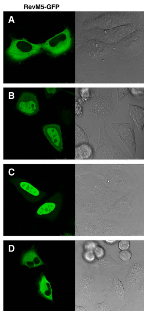
Figure 2. Effect of 3-(5-phenyltetrazol-2-yl)acrylic acid ethyl esters on the localization of RevM5-GFP in living cells. HeLa cells expressing RevM5-GFP were incubated with test compound. Two hours after addition of the compounds, the cells were analyzed by fluorescence microscopy. The left panels are the fluorescent images and the right panels the corresponding differential interference contrast images. RevM5-GFP before addition of compound is localized in the cytoplasm (A). Addition of 25 nM LMB (B) or 10 µg/ml (36 µM) 7d-cis (C) resulted in a predominant nuclear localization of the RevM5-GFP, while 10 µg/ml 6d (D) had no effect on the localization of RevM5-GFP.
