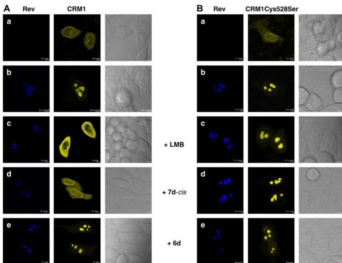
Figure 4. 3-(5-Phenyltetrazol-2-yl)acrylic acid ethyl esters interfere with the co-localization of Rev-BFP and CRM1-EYFP in living cells but not with the co-localization of the Rev-BFP and EYFP-CRM1Cys528 mutant. (A) HeLa cells expressing Rev-BFP or/and CRM1-EYFP were analyzed by fluorescence microscopy. Rev-BFP localizes in the nucleoli of the cells (b, left panel), while CRM1-EYFP is found at the nuclear rim (a, middle panel). In cells co-expressing both Rev-BFP and CRM1-EYFP, CRM1 colocalizes with Rev-BFP in the nucleoli (b, middle panel). Two hours after addition of compound the co-localization of CRM1-EYFP with Rev-BFP was analyzed (c: LMB; d: 7d-cis ; e: 6d ). (B) Similar as in (A) but with a mutant CRM1-EYFP with a serine at position 528 instead of cysteine.
