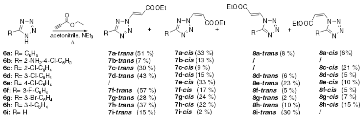
Scheme 3: condensation reaction of 5-aryltetrazoles 6 with ethyl propiolate
