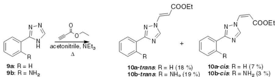
Scheme 4: condensation reaction of 3-aryl-1,2,4-triazole 9 with ethyl propiolate
