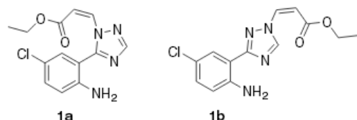
Figure 1. Erroneous ( 1a ) and revised ( 1b ) structure of PKF050-638.
