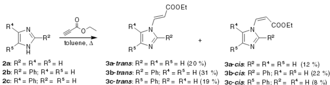
Scheme 1: condensation reaction of imidazole 2 with ethyl propiolate
