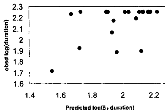
Figure 5. (a) GOLPE model, using compounds 1–24, alkyl hydroxyl GRID probe, block-scaled with \log D_{7.4} , variable reduction from 12168 variables to 188 using D-optimal selection followed by Full Factorial Design selection. Blue fields represent negative coefficients, good positions to place hydrogen binding groups, poor places to place steric bulk; yellow fields, good places for steric bulk, poor places for hydrogen binding interactions. (b) Duration predictions from the GOLPE model for 23 subsequently synthesized compounds.
