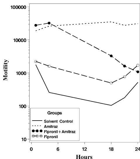
Fig. 5. Geometric means of motility assay calculated over all doses for unstimulated ticks through time.
