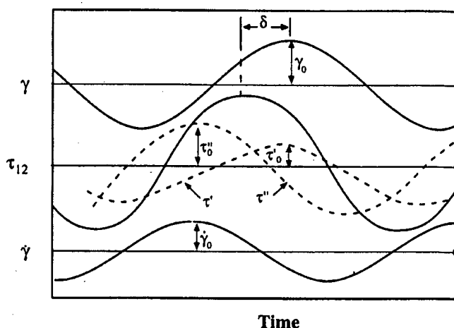
Figure 3.3.3. Sinusoidally oscillating shear strain produces a sinusoidal stress phase shifted by an amount \delta . For analysis the stress wave is broken down into two waves, \tau' in phase with \gamma and \tau'' 90° out of phase. Note that \tau'' is in phase with the rate of strain wave \dot{\gamma} = d\gamma/dt .
