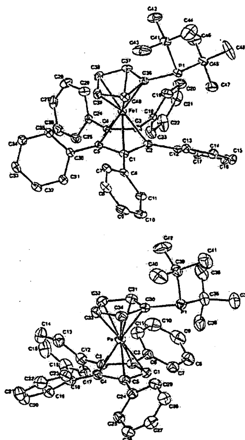
FIGURE 1. ORTEP diagrams of \text{Ph}_3\text{FcP}(\text{t-Bu})_2 and \text{Ph}_3\text{FcP}(\text{t-Bu}) .
