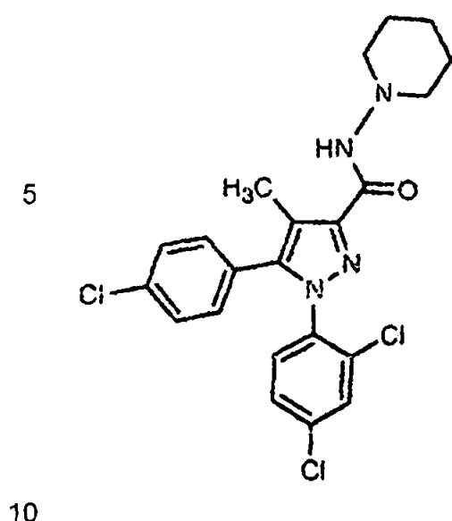
SR 141716
