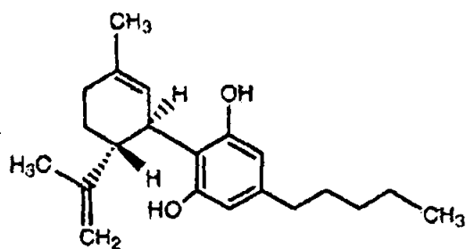
CANNABIDIOL
