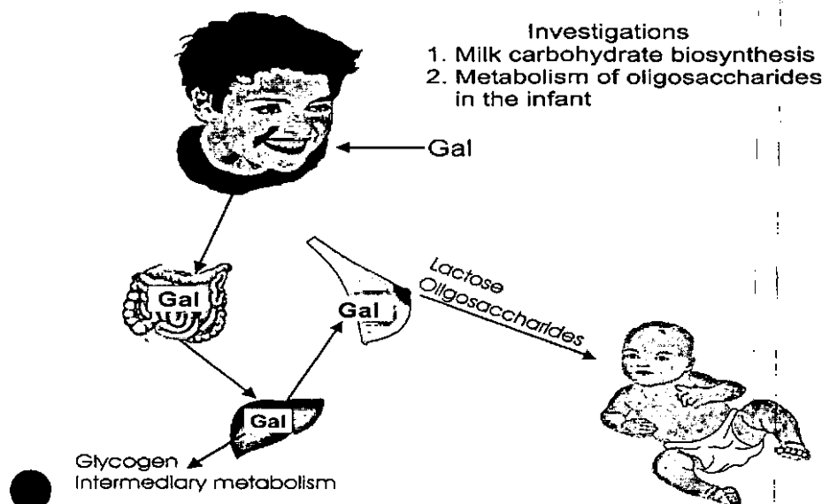
Figure 1 Scheme of our studies with ^{13}\text{C} -labeled monosaccharides ( [^{13}\text{C}]\text{Gal} and [^{13}\text{C}]\text{Glc} ) to investigate questions with regard to milk carbohydrate biosynthesis and oligosaccharide metabolism in the infant.
