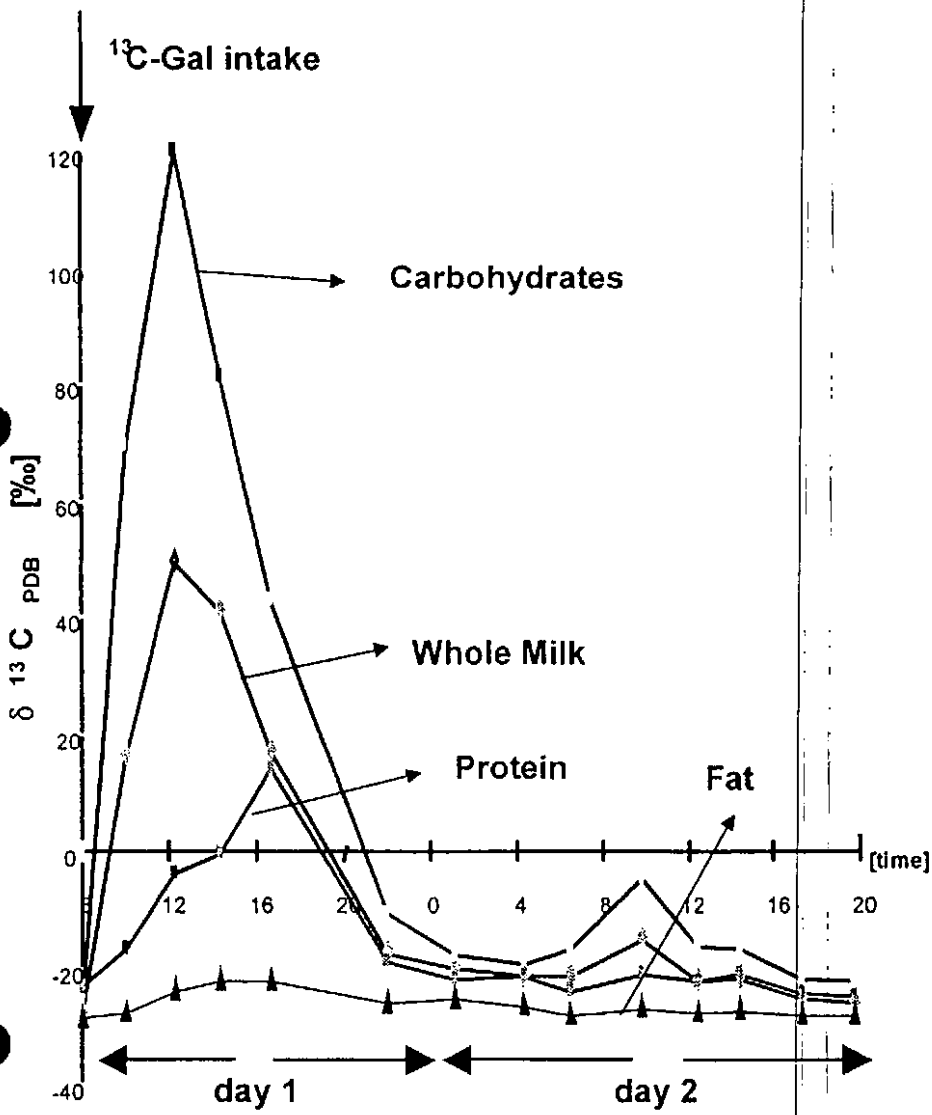
Figure 2 13 C enrichment (expressed as \delta^{13}\text{C}_{\text{PDB}} [‰]) of whole milk and milk fractions from one woman during the first 36 h after administration of a single oral Gal bolus (25 g of Gal plus 2 g of [ 13 C]Gal; D-Gal; 1- 13 C, 99%).
