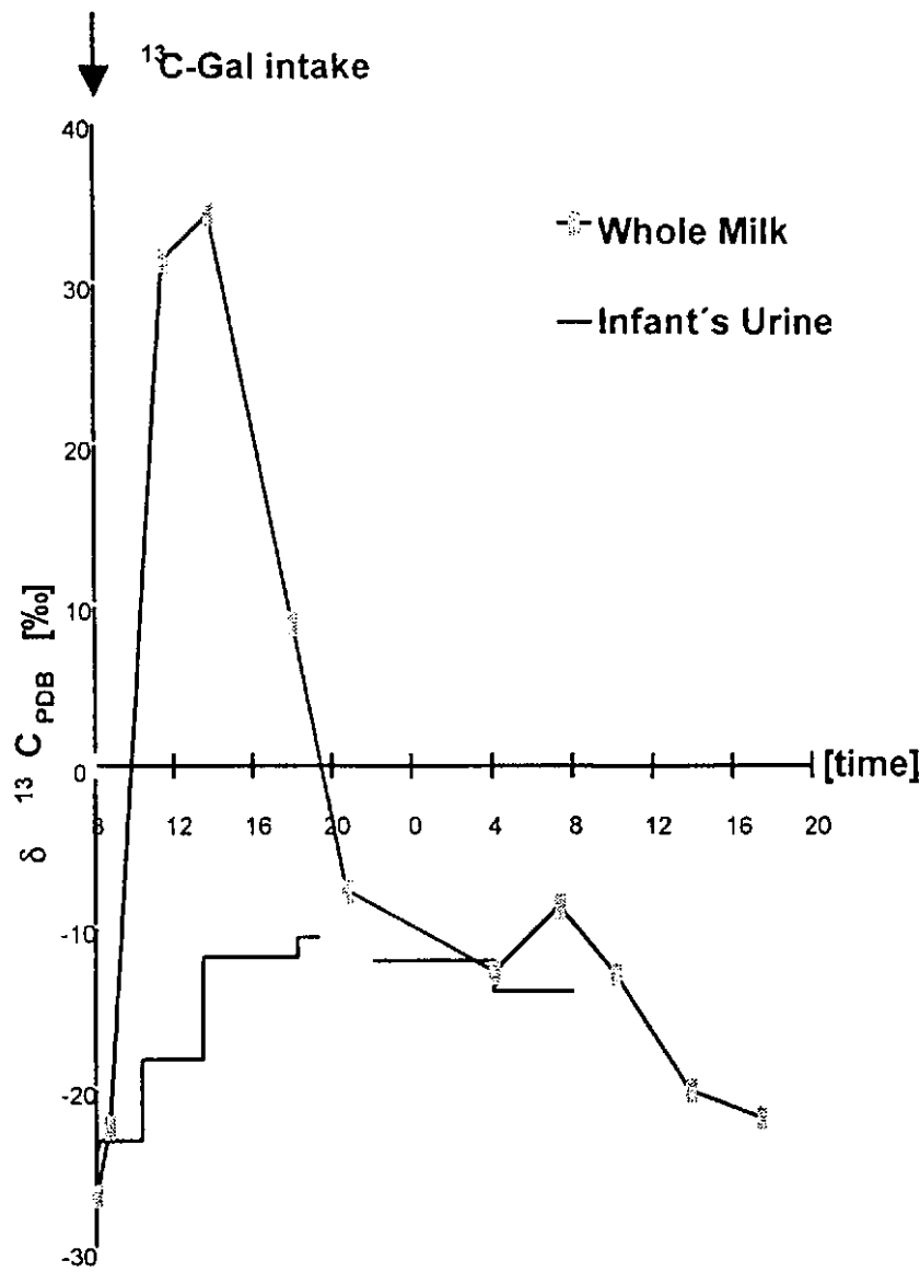
Figure 4 13 C enrichment in mother's whole milk and in urine of her infant.
