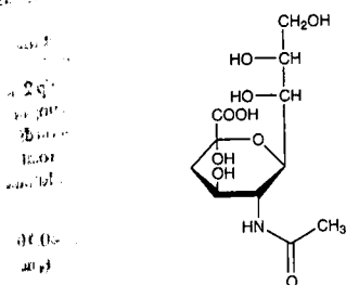
N-Acetylneuraminic acid
