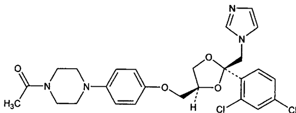
Relative stereochemistry
