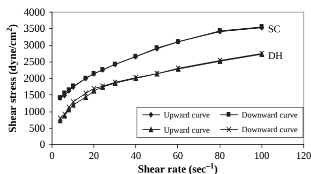
FIGURE 4. Flow curves of 3% CP 934 gels containing secnidazole (SC) or doxycycline hydrochloride (DH) at 25°C.
