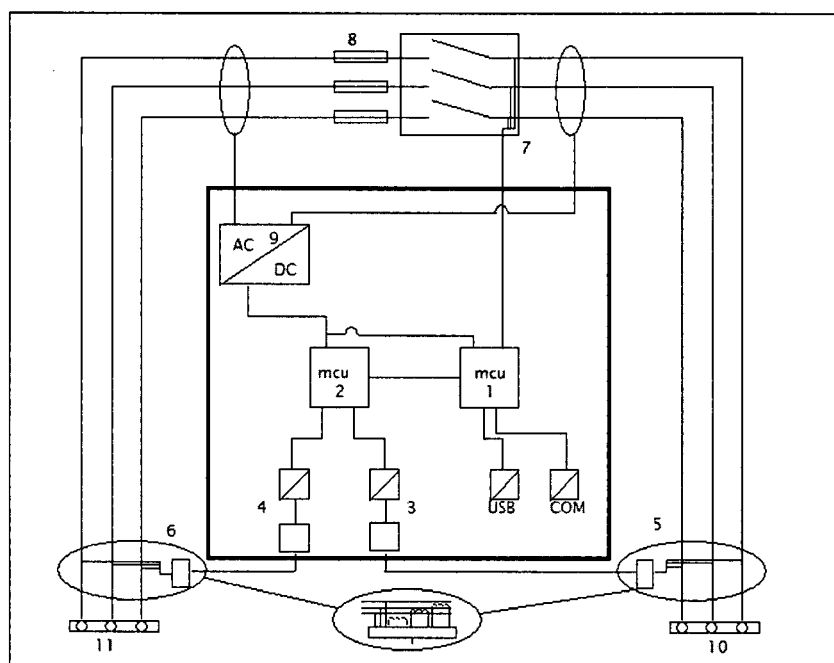
Figura 2. Gabinete Control Red
