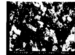
(a) sludge: 20%, nano-SiO 2 : 0%, 1 day
