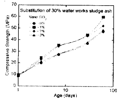
Figure 9. Influence of both 30% sludge ash and nano-SiO 2 on the compressive strengths of paste samples.
