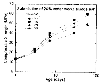
Figure 8. Influence of both 20% sludge ash and nano-SiO 2 on the compressive strengths of paste samples.
