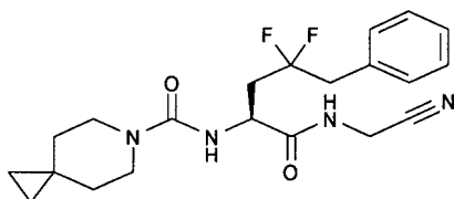
15 N-[(S)-1-(cianometilcarbamoil)-4-ciclopropil-3,3-difluorobutil]-6-aza-espiro[2.5]octano-6-carboxamida
