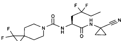
15 N-[(S)-1-(1-cianociclopropilcarbamoil)-4-ciclopropil-3,3-difluorobutil]-1,1-difluoro-6-azaespiro[2.5]octano-6-carboxamida
