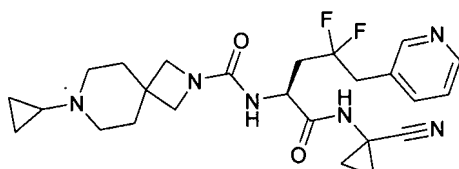
5 N-[(S)-1-(1-cianociclopropilcarbamoil)-3,3-difluoro-4-piridin-4-ilbutil]-7-ciclopropil-2,7-diazaespiro[3.5]nonano-2-carboxamida
