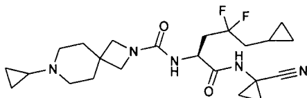
N-[(S)-1-(cianometilcarbamoil)-3,3-difluoro-4-fenilbutil]-7-ciclopropil-2,7-diazaespiro[3.5]nonano-2-carboxamida
