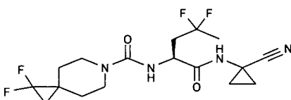
10 N-[(S)-1-(1-cianociclopropilcarbamoil)-3,3-difluoropentil]-1,1-difluoro-6-azaespiro[2.5]octano-6-carboxamida
