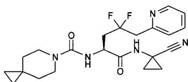
5 N-[(S)-1-(1-cianociclopropilcarbamoil)-3,3-difluoro-4-piridin-3-ilbutil]-6-aza-espiro[2.5]octano-6-carboxamida
