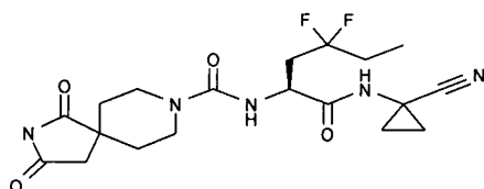
15 N-[(S)-1-(1-cianociclopropilcarbamoil)-3,3-difluoropentil]-1,3-dioxo-2,8-diazaespiro[4.5]decano-8-carboxamida
