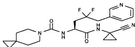
N-[(S)-1-(1-cianociclopropilcarbamoil)-3,3-difluoro-4-piridin-4-ilbutil]-6-aza-espiro[2.5]octano-6-carboxamida
