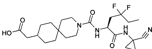
15 N-[(S)-1-(1-cianociclopropilcarbamoil)-3,3-difluoropentil]-1,3-dioxo-2,8-diazaespiro[4.5]decano-8-carboxamida
