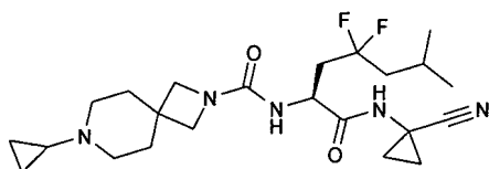
N-[(S)-1-(1-cianociclopropilcarbamoil)-4-ciclopropil-3,3-difluorobutil]-7-ciclopropil-2,7-diazaespiro[3.5]nonano-2-carboxamida
