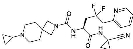
N-[(S)-1-(1-cianociclopropilcarbamoil)-3,3-difluoro-4-piridin-3-ilbutil]-7-ciclopropil-2,7-diazaespiro[3.5]nonano-2-carboxamida
