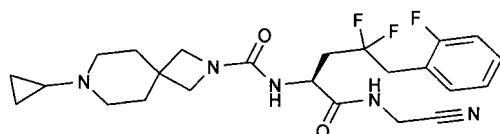
N-[(S)-1-(1-cianociclopropilcarbamoil)-3,3-difluorobutil]-1,1-difluoro-6-azaespiro[2.5]octano-6-carboxamida
