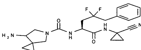
15 N-[(S)-1-(1-cianociclopropilcarbamoil)-3,3-difluoro-4-fenilbutil]-7-dimetilamino-5-azaespiro[2.4]heptano-5-carboxamida
