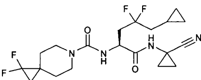
N-[(S)-1-(1-cianociclopropilcarbamoil)-3,3-difluoro-4-piridin-3-ilbutil]-1,1-difluoro-6-azaespiro[2.5]octano-6-carboxamida
