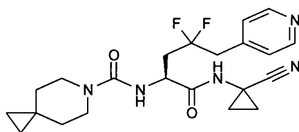
10 N-[(S)-1-(cianometilcarbamoil)-3,3-difluoro-4-fenilbutil]-6-azaespiro[2.5]octano-6-carboxamida
