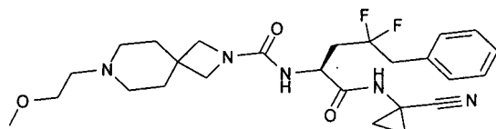
N-[(S)-1-(1-cianociclopropilcarbamoil)-3,3-difluoro-4-fenilbutil]-9-(2-metoxietil)-3,9-diazaespiro[5.5]undecano-3-carboxamida
