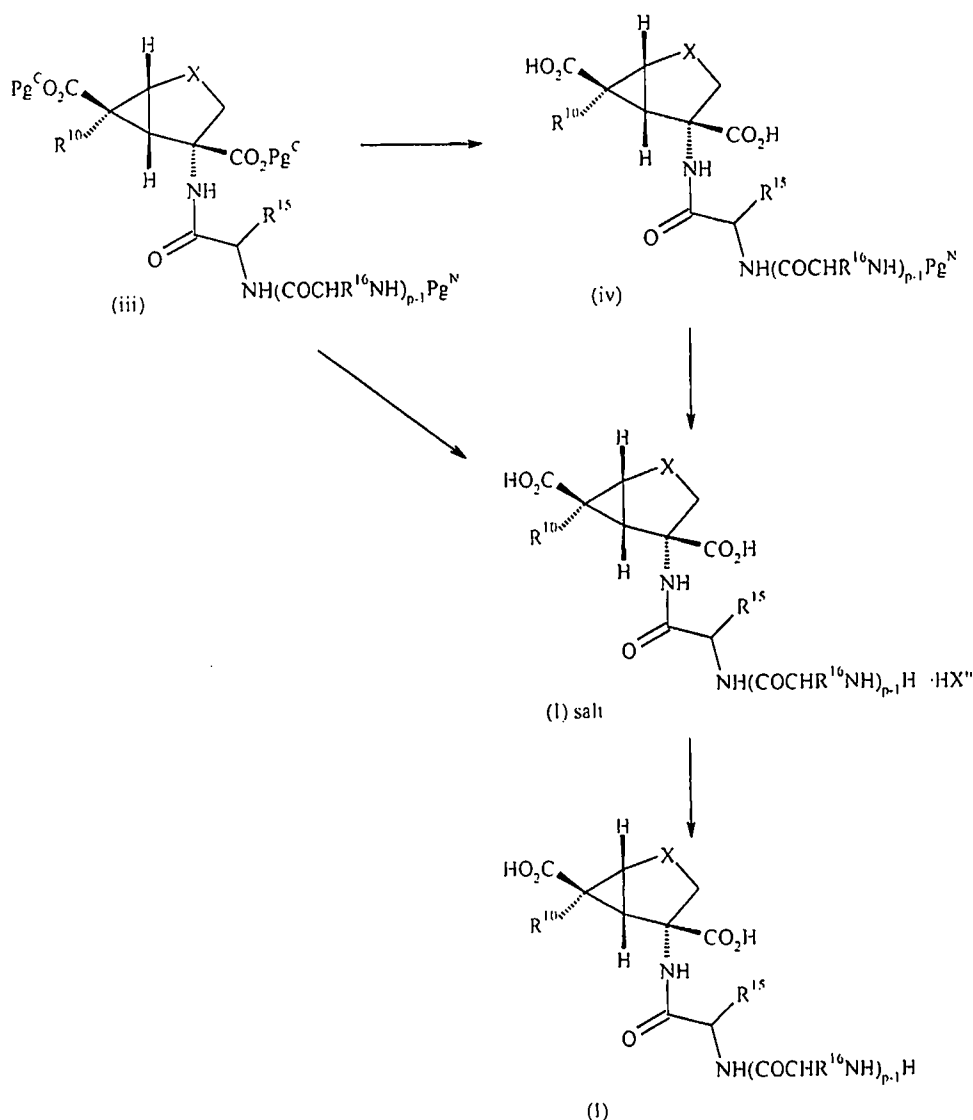
Scheme 2
