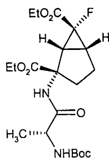
Isomer A
