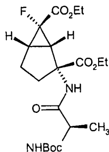
Isomer B
