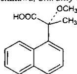
(R)-(-)-form
