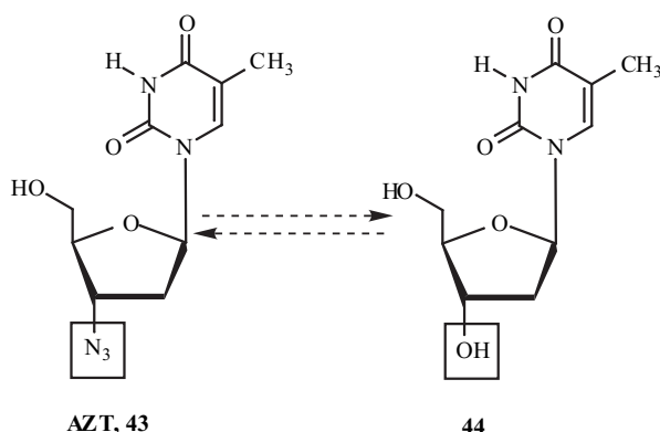
Scheme 11.
