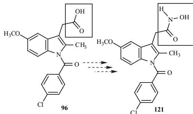
Scheme 38.
