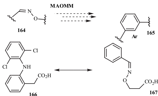
Scheme 55.
