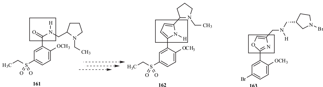
Scheme 54..
