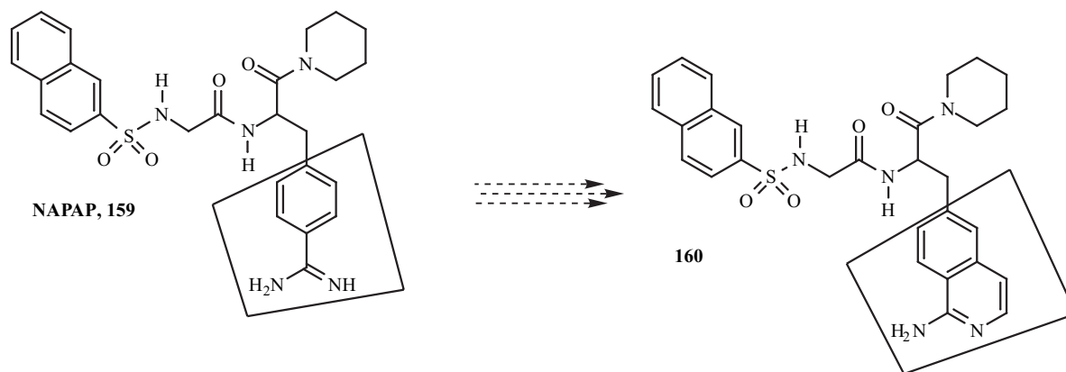
Scheme 53.
