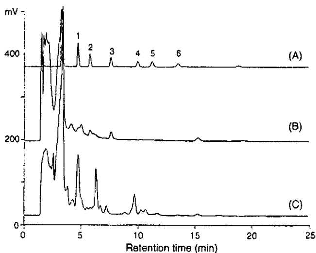
Fig. 1. HPLC chromatograms for analysis of aldehydes in excipients after derivatization with DNPH. Method conditions are shown in Section 2.5. (A) Method standard containing 1.0 mg/mL levels of C_1 – C_6 aldehydes. (B) A sample of hydroxypropyl cellulose. (C) A sample of hypromellose. Peaks: 1 = formaldehyde, 2 = acetaldehyde, 3 = propanal, 4 = butanal, 5 = pentanal, 6 = hexanal.
