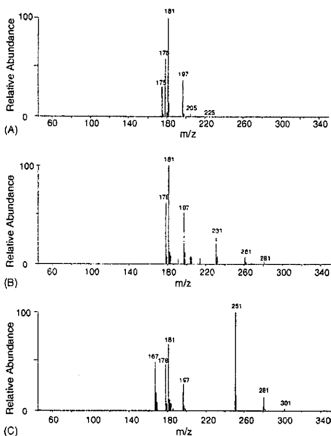
Fig. 4. Negative ion chemical ionization mass spectra of PFBHA aldehyde oximes. Method conditions are shown in Section 2.3. (A) Formaldehyde-PFBHA oxime. (B) Pentanal-PFBHA oximes. (C) Benzaldehyde-PFBHA oximes.
