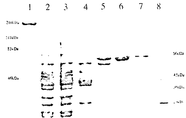
FIG. 4. SDS-PAGE analysis of the purification of cocaine esterase to homogeneity. Lane 1, molecular weight marker; lane 2, molecular weight marker; lane 3, molecular weight marker; lane 4, molecular weight marker; lane 5, molecular weight marker; lane 6, molecular weight marker; lane 7, molecular weight marker; lane 8, purified cocaine esterase. The
