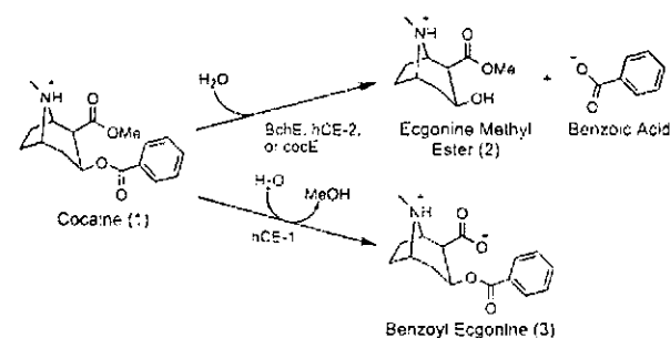
Fig. 1 Cocaine hydrolysis. Both the benzoyl ester and the methyl ester of cocaine (1) can be hydrolyzed by different enzymes to give nonpsychoactive metabolites ecgonine methyl ester (2) and benzoyl ecgonine (3). Human liver esterases hCE-1 and hCE-2, and the serum esterase butyrylcholinesterase BchE account for the ~30 min in vivo half-life of cocaine. CocE hydrolyzes the benzoyl ester of cocaine to form ecgonine methyl ester (2) and benzoic acid.
