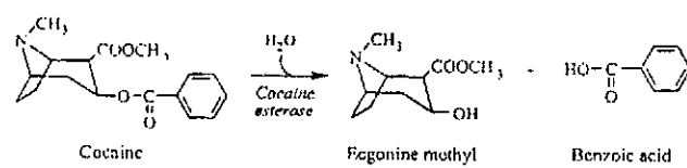
FIG. 1. Cocaine esterase reaction.
