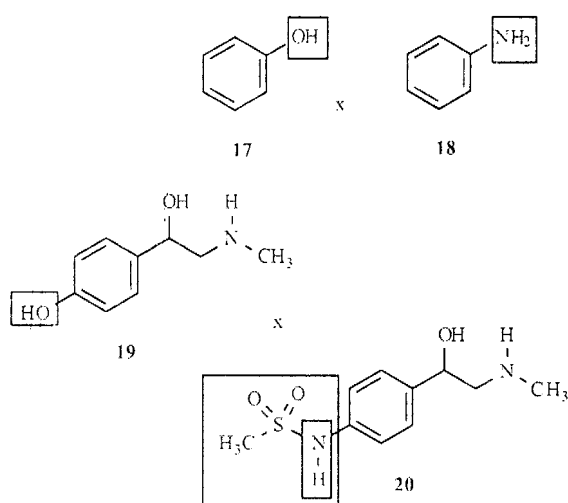
Scheme 3.
