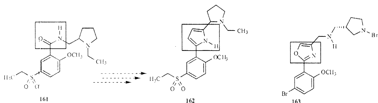
Scheme 54.
