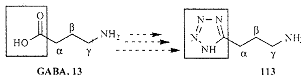
Scheme 36.
