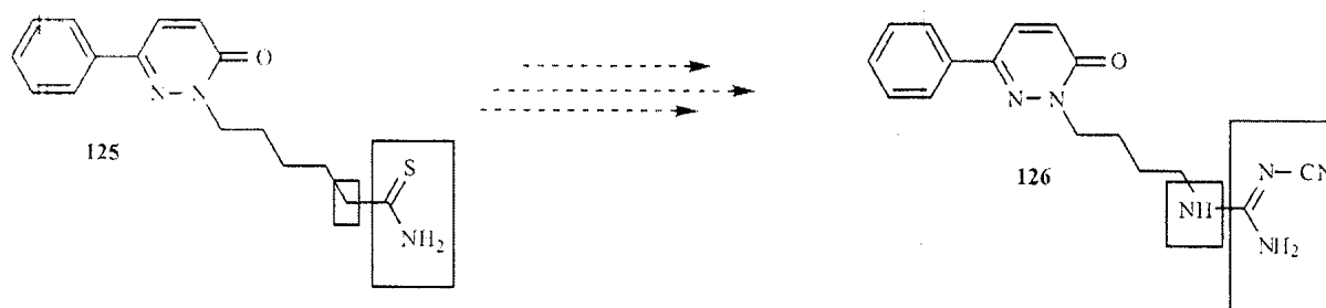
Scheme 41.
