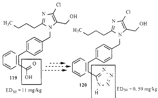
Scheme 37.
