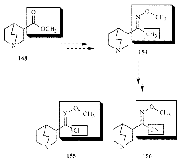
Scheme 51.
