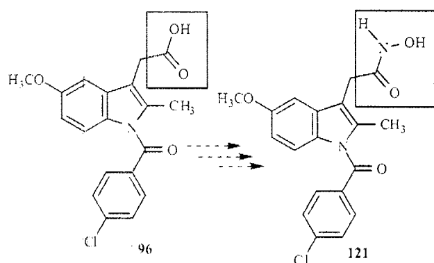
Scheme 38.
