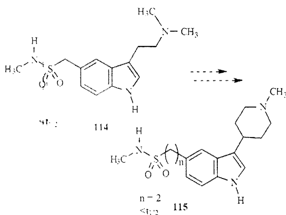
Scheme 34.
