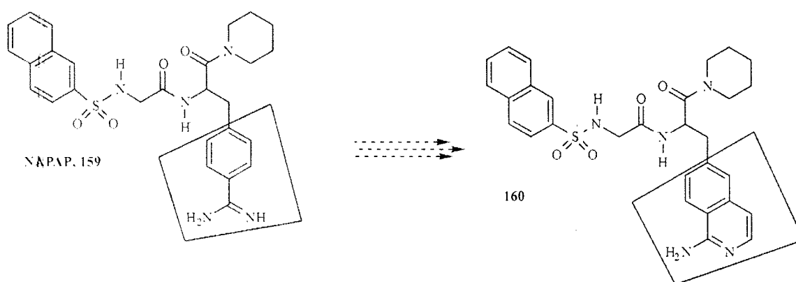
Scheme 53.
