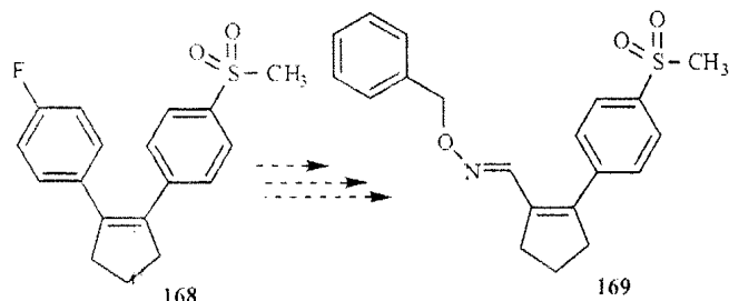
Scheme 56.
