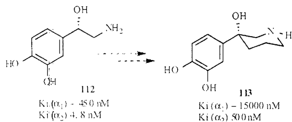
Scheme 33.
