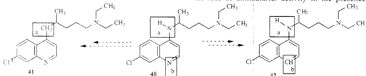
Scheme 10.
