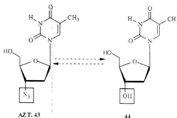
Scheme 11.
