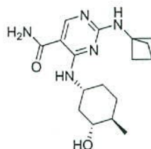
2-((bicyclo[1.1.1]pentan-1-ylamino)-4-(((1R,3R,4R)-3-hidroxi-4-metilciclohexil)amino)pirimidina-5-carboxamida,
