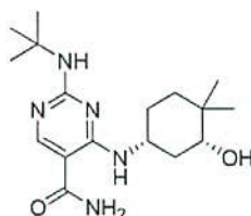
2-( tert -butilamino)-4-(((1R,3R)-3-hidroxi-4,4-dimetilciclohexil)amino)pirimidina-5-carboxamida,
