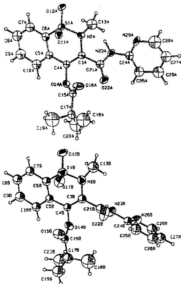
Fig. 3. Conformations of the two independent molecules of paroxetene pivalate (I) in polymorph 2. Thermal ellipsoids are drawn at the 40% probability level, and H atoms are shown as spheres of arbitrary size ([40], reproduced with the permission of the American Pharmaceutical Association).
