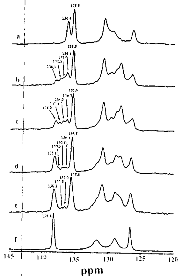
Fig. 9. Resonance signals of the phenyl carbon (C-15) attached to the side chain in the ^{13}\text{C} -CP-MAS NMR spectra of neotame anhydrate: (a) sample generated by placing the original monohydrate under vacuum ( < 1 Torr) for 3 days; (b–e) sample after being sealed in a jar for 2, 4, 6 and 8 days, respectively; (f) sample after being exposed to a relative humidity environment of 84% for 12 days ([29], reproduced with the permission of the American Chemical Society).
