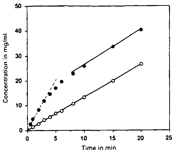
Fig. 6. Concentration profile during intrinsic dissolution of anhydrous and monohydrate theophylline from a disk at 23°C: ●, anhydrous; ○, monohydrate. (Reproduced from Ref. [16] with the permission of the copyright owner, Marcel Dekker, New York, USA.)
