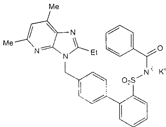
Fig. 6. The molecular structure of the angiotensin-II antagonist MK-996.
