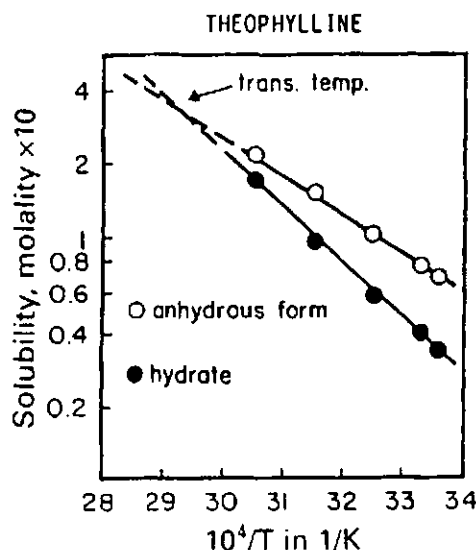
Fig. 4. van't Hoff-type plot of molal solubility (mol kg -1 , log scale) against the reciprocal of the absolute temperature for the anhydrous and hydrated forms of theophylline in water. (Reproduced from Ref. [4] with the permission of the copyright owner, American Pharmaceutical Association, Washington DC, USA.)
