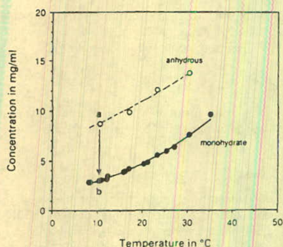
Fig. 3 Solubility dependence on temperature, for anhydrous and monohydrate theophylline in phosphate buffer (pH 6). Points a and b represent the concentration range in which the phase transformation was studied. (Reproduced from Ref. [11] with the permission of the copyright owner, Elsevier Publishers B.V., Amsterdam, Netherlands.)
