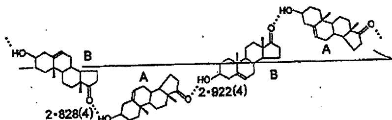
Fig. 10. Head-to-tail hydrogen bonding in Form I of dehydroepiandrosterone. A and B are crystallographically distinct and distances are in Å
