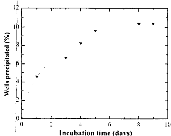
Fig. 2. Typical rate of appearance of solids during a thermally driven HT crystallization experiment [63].
