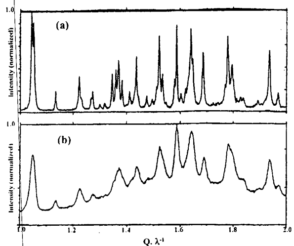
Fig. 8. A partial comparison of (a) a synchrotron pattern of polymorph II of roxifiban, collected using a wavelength of 1.00006 Å with (b) a conventional X-ray diffraction pattern using \text{CuK}\alpha radiation in a region where there are many overlapping peaks. The patterns are plotted as a function of Q = 2\pi/d = 4\pi \sin \theta/\lambda to remove the effects of different wavelengths ([61], reproduced with the permission of the American Pharmaceutical Association).
