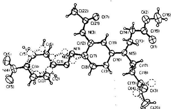
Fig. 5. ORTEP plots of the two molecular conformations (1 and 2) for the X-ray structure determination of 2'-acetamido-4'-[ N,N -bis(2-methoxycarbonyl)ethylethyl]amino]-4-nitroazobenzene (Scheme 1 Structure) at 293 K. Thermal ellipsoids are shown at 30% for clarity, with conformer 2 being represented by the solid lines and Conformer 1 by the dotted lines ([48], reproduced with the permission of the American Chemical Society).
