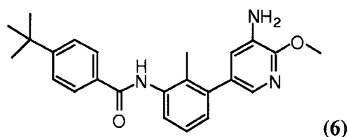
N -(3-(5-Amino-6-methoxypyridin-3-yl)-2-methylphenyl)-4- tert -butylbenzamide (6)
