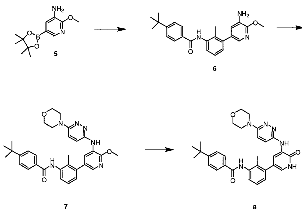
N -(3-(5-Amino-6-methoxypyridin-3-yl)-2-methylphenyl)-4- tert -butylbenzamide (6)
