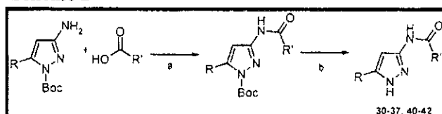
Scheme 2 a
