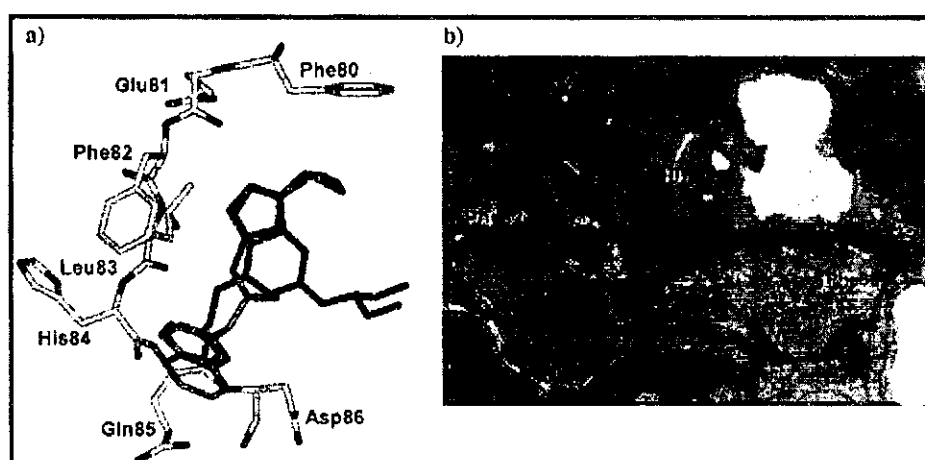
Figure 3. Crystal structure of 41 in complex with CDK2/cyclin A: (a) overlap of 41 (atom-type colored) and roscovitine (magenta) complexed to CDK2/cyclin A; (b) surface representation of ATP binding cleft, colored by residue hydrophobicity, in complex with 41 . Red indicates most hydrophobic residues, and blue indicates the most polar ones.
