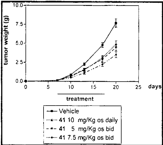
Figure 6. Antitumor efficacy of 41. Compound 41 shows a 53% tumor growth inhibition (TGI) against a human ovarian cancer model (A2780) transplanted into nude mice when administered at 7.5 mg/kg twice a day for 10 consecutive days.
