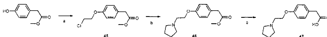
Scheme 5 a
