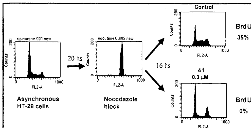
Figure 4. 41 blocks cell cycle progression. Cells synchronized in G2/M by nocodazole treatment were released in the absence or in the presence of 41. In comparison with the control cells, cells treated with 41 showed a block in G1 and a complete absence of S phase, as confirmed by the lack of BrdU incorporation.
