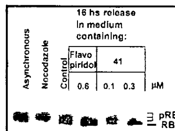
Figure 5. 41 blocks pRb phosphorylation. After the treatment with 0.3 \mu M 41, the substrate retinoblastoma protein (pRb) is mainly in the dephosphorylated form.
