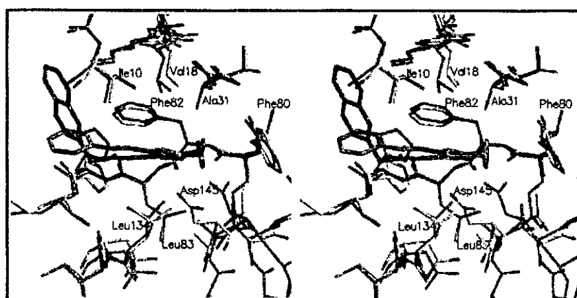
Figure 2. Stereoview showing the structure of CDK2 complexed with compound 4 (green carbon atoms for the protein, cyan carbon atoms for the inhibitor) superimposed on the structure of CDK2/cyclin A with compound 41 (yellow carbon atoms for the protein, orange for the inhibitor). It is clear from this figure that compound 41 retains the same hydrogen-bonding pattern as observed for 4 . The benzylic methylene of the naphthylacetamide group of 41 with respect to the benzoic group of 4 allows this substituent to adopt a bent conformation with the naphthyl group packing onto Ile10. The differences in the conformations of the protein residues are caused by having cyclin bound in one case and not in the other. This does not appear to affect the binding of the ligand.
