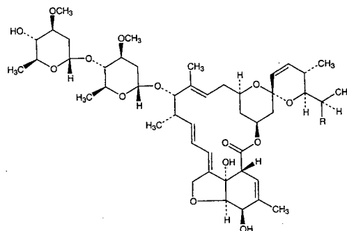
component B 1b , R = CH 3
