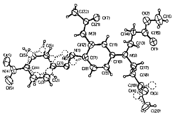
Fig. 5. ORTEP plots of the two molecular conformations (1 and 2) for the X-ray structure determination of 2'-acetamido-4'-[ N,N -bis(2-methoxycarbonyl)ethyl]amino]-4-nitroazobenzene (Scheme 1 Structure) at 293 K. Thermal ellipsoids are shown at 30% for clarity, with conformer 2 being represented by the solid lines and Conformer 1 by the dotted lines ([48], reproduced with the permission of the American Chemical Society).
