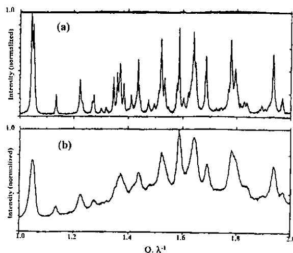
Fig. 8. A partial comparison of (a) a synchrotron pattern of polymorph II of roxifiban, collected using a wavelength of 1.00006 \text{ \AA} with (b) a conventional X-ray diffraction pattern using \text{CuK}\alpha radiation in a region where there are many overlapping peaks. The patterns are plotted as a function of Q = 2\pi/d = 4\pi \sin \theta/\lambda to remove the effects of different wavelengths ([61], reproduced with the permission of the American Pharmaceutical Association).
