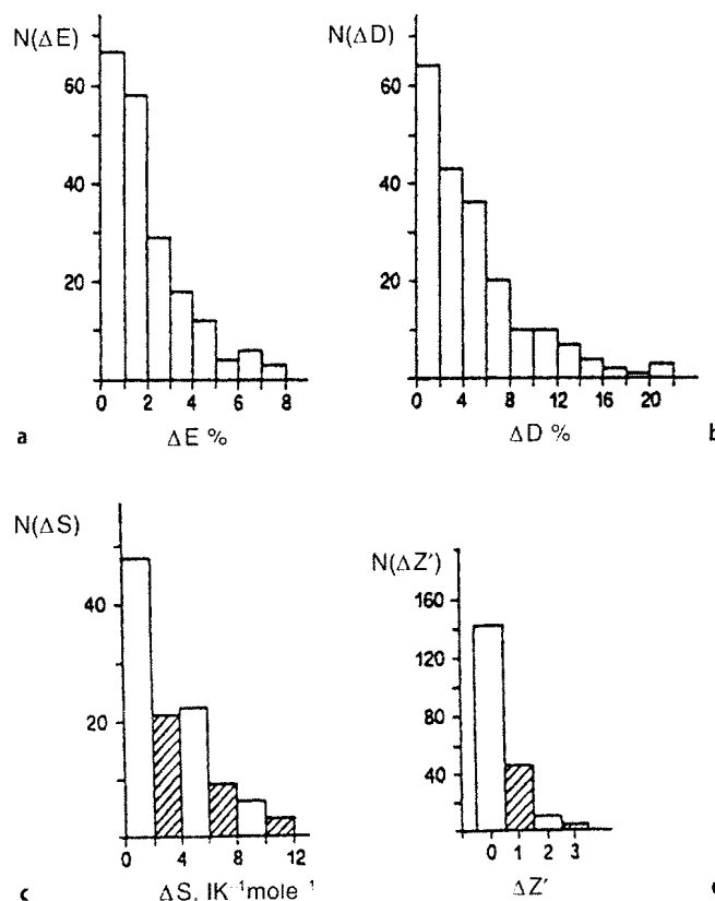
Fig. 6a–d. Histograms of differences in properties between polymorphs: a \Delta E (packing energy, %); b \Delta D (density, %); c \Delta S (lattice-vibrational entropy, \text{J K}^{-1} \text{mol}^{-1} ); d \Delta Z' (no. of molecules in the asymmetric unit). (Reprinted with permission from [79], copyright 1995, American Chemical Society)
