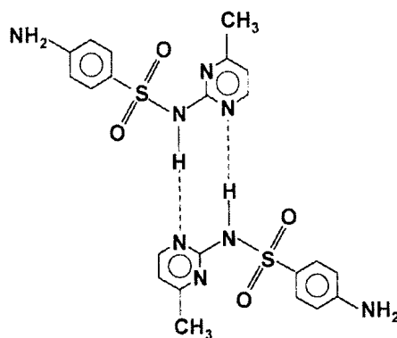
Fig. 9. Schematic representation of the hydrogen bonded dimer occurring in two polymorphs of sulphamerazine
