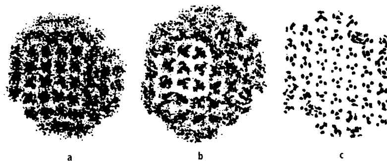
Fig. 2a–c. Images of a crystalline cluster of t -butyl chloride molecules at various stages of cooling, looking down the threefold molecular axis: a orientationally disordered tetragonal phase at 130 K; b nucleus of monoclinic phase growing in tetragonal phase at 80 K; c ordered monoclinic phase at 50 K after transformation. Surface molecules tend to be disordered at all temperatures. (Reprinted with permission from [44], copyright 1995 American Chemical Society)
